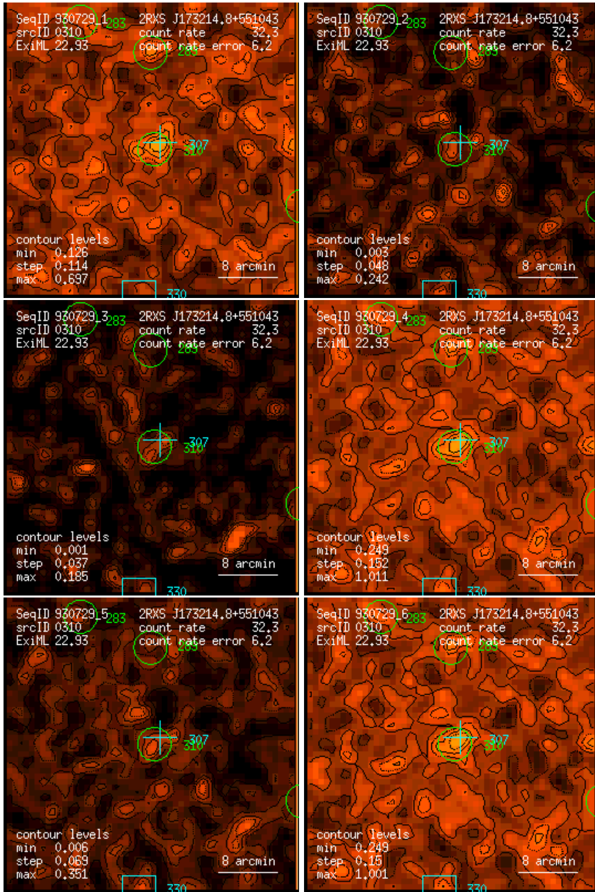
Figure 310: RASS 930729: detection 0310: band rate images, Gaussian filter: (1) PSPC channels 11 – 41, (2) 52 – 90, (3) 91 – 201, (4) 11 – 235, (5) 52 – 201, (6) 11 – 201. Broad band rates in counts/ks. Band rate contour levels in counts/ks/arcmin 2 .
