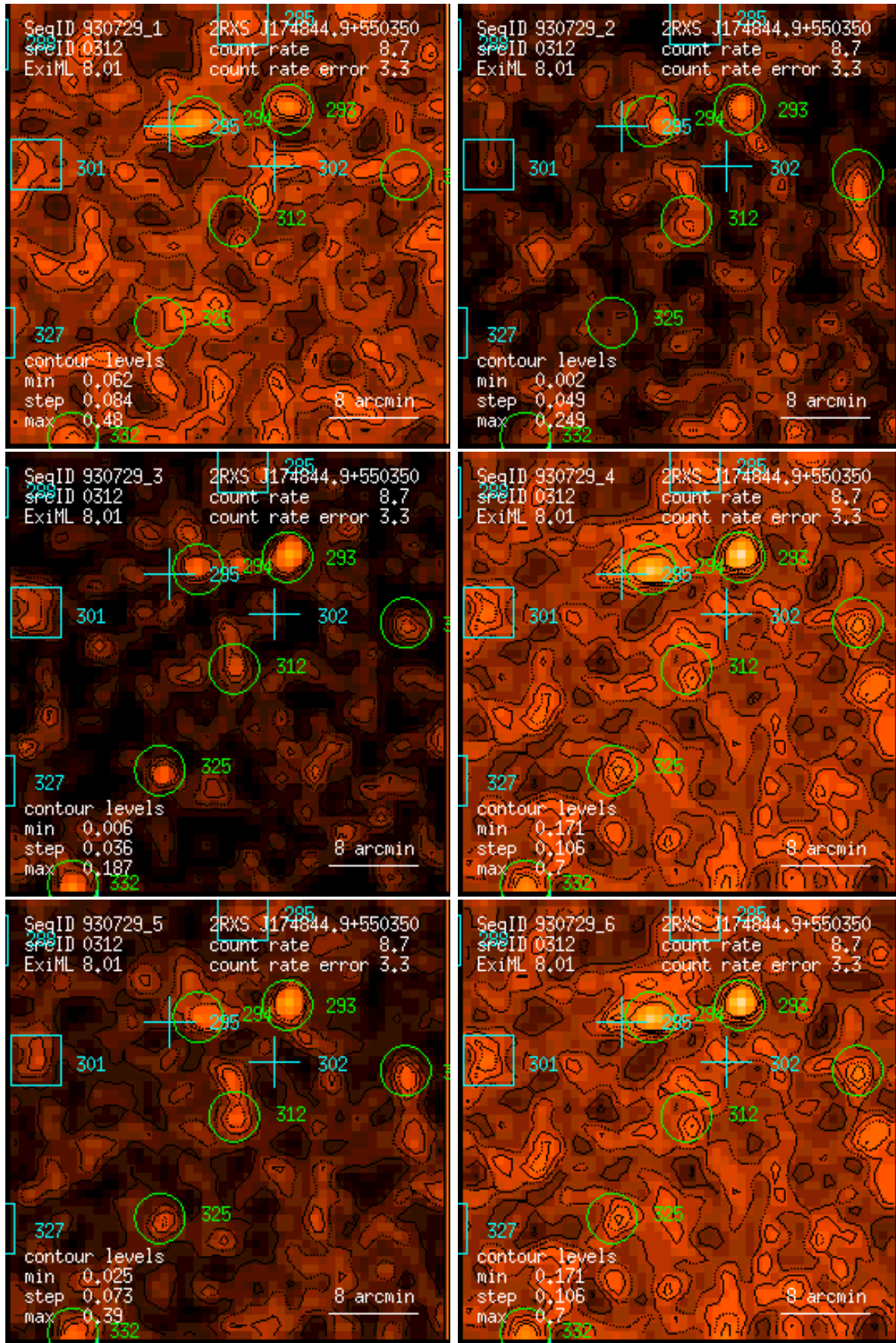
Figure 312: RASS 930729: detection 0312: band rate images, Gaussian filter: (1) PSPC channels 11 – 41, (2) 52 – 90, (3) 91 – 201, (4) 11 – 235, (5) 52 – 201, (6) 11 – 201. Broad band rates in counts/ks. Band rate contour levels in counts/ks/arcmin 2 .
