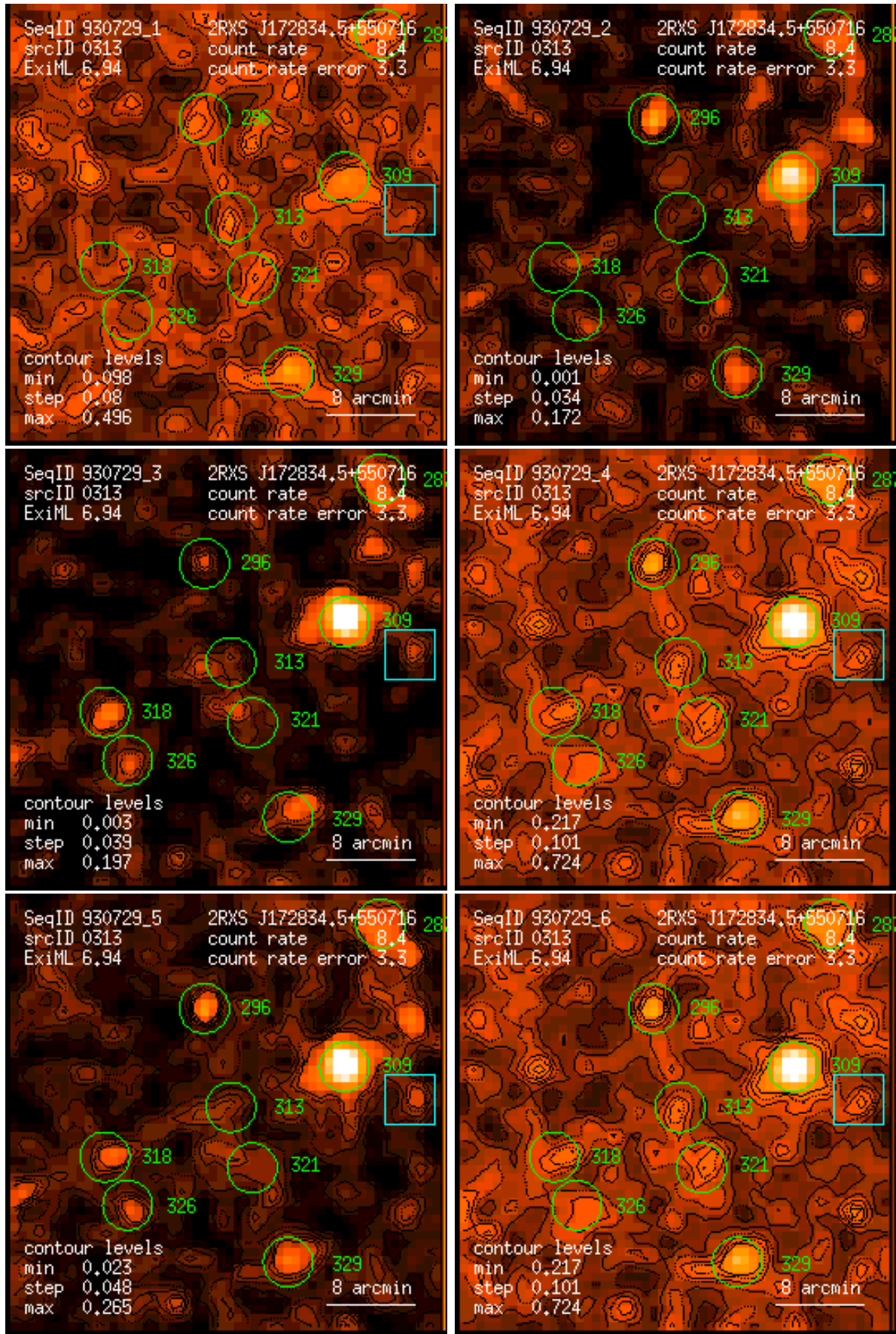
Figure 313: RASS 930729: detection 0313: band rate images, Gaussian filter: (1) PSPC channels 11 – 41, (2) 52 – 90, (3) 91 – 201, (4) 11 – 235, (5) 52 – 201, (6) 11 – 201. Broad band rates in counts/ks. Band rate contour levels in counts/ks/arcmin 2 .
