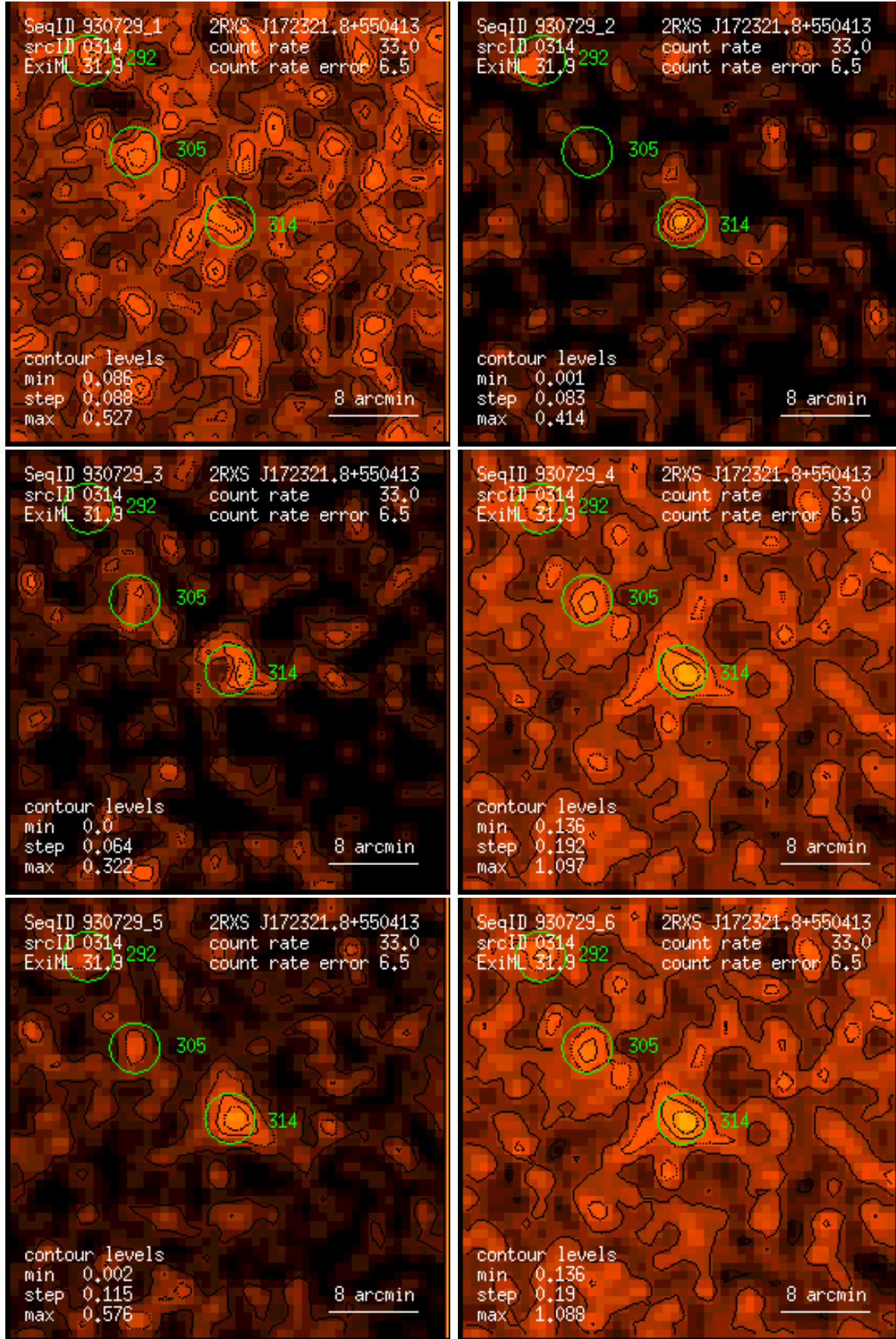
Figure 314: RASS 930729: detection 0314: band rate images, Gaussian filter: (1) PSPC channels 11 – 41, (2) 52 – 90, (3) 91 – 201, (4) 11 – 235, (5) 52 – 201, (6) 11 – 201. Broad band rates in counts/ks. Band rate contour levels in counts/ks/arcmin 2 .
