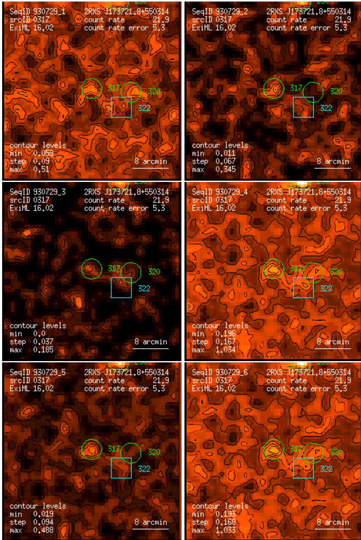
Figure 317: RASS 930729: detection 0317: band rate images, Gaussian filter: (1) PSPC channels 11 – 41, (2) 52 – 90, (3) 91 – 201, (4) 11 – 235, (5) 52 – 201, (6) 11 – 201. Broad band rates in counts/ks. Band rate contour levels in counts/ks/arcmin 2 .
