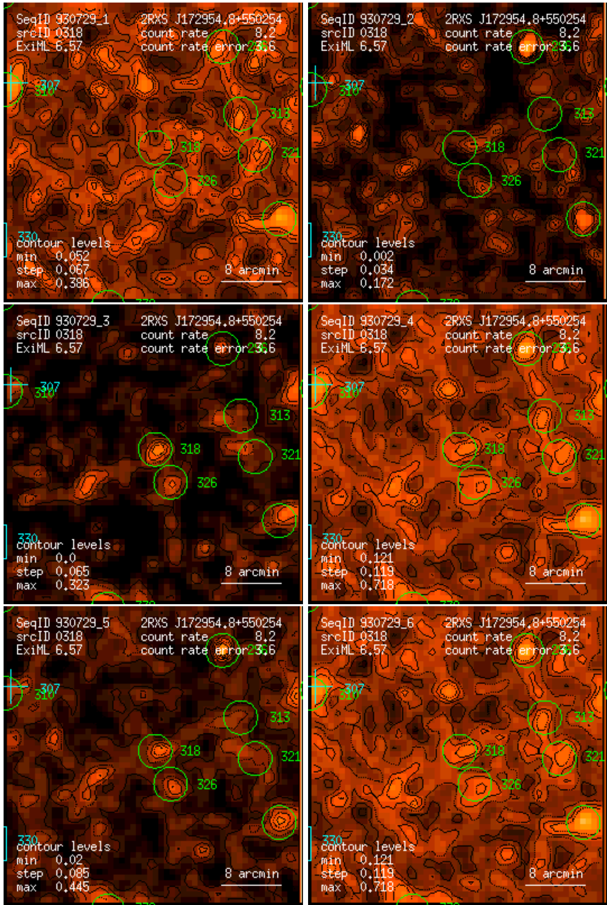
Figure 318: RASS 930729: detection 0318: band rate images, Gaussian filter: (1) PSPC channels 11 – 41, (2) 52 – 90, (3) 91 – 201, (4) 11 – 235, (5) 52 – 201, (6) 11 – 201. Broad band rates in counts/ks. Band rate contour levels in counts/ks/arcmin 2 .
