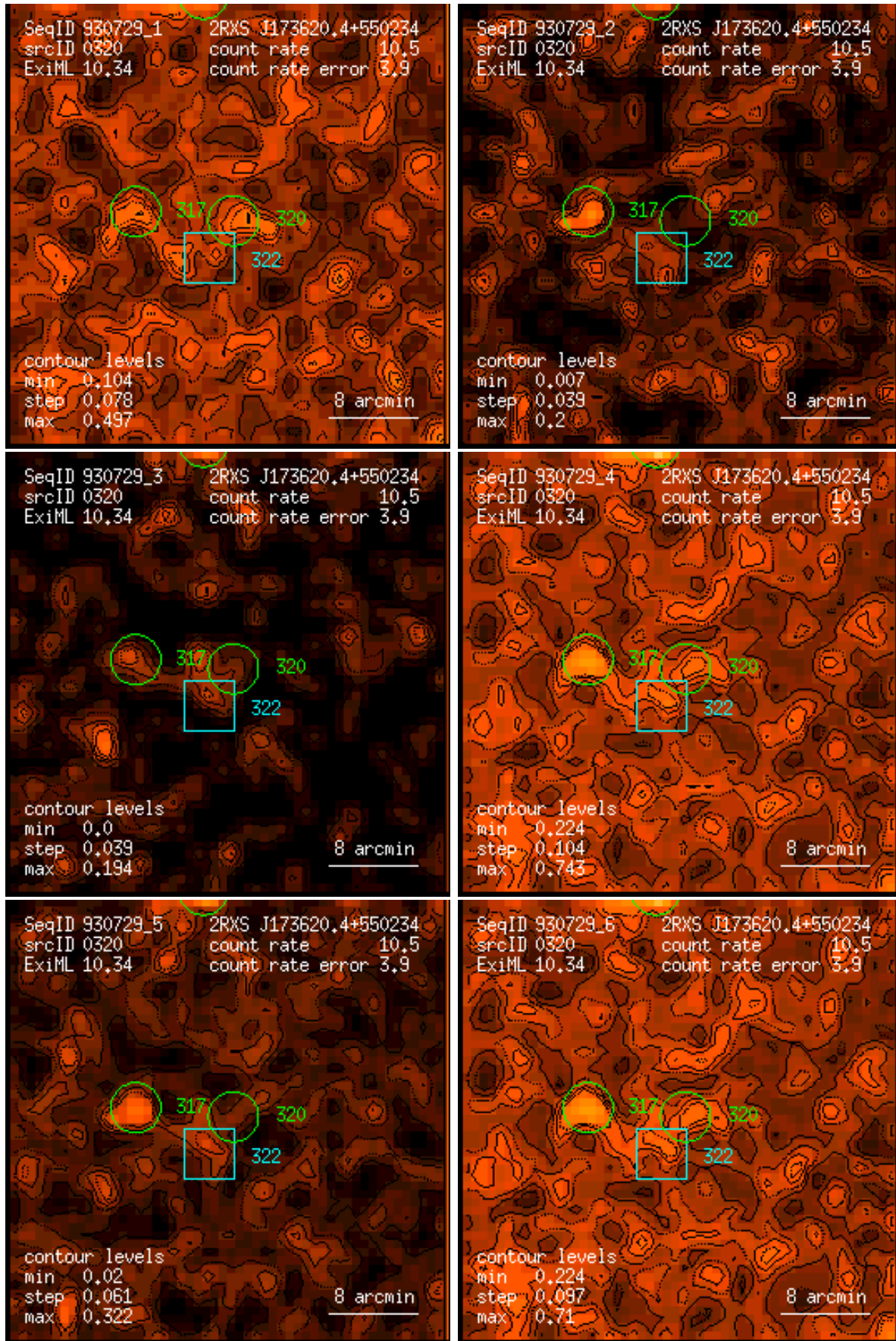
Figure 320: RASS 930729: detection 0320: band rate images, Gaussian filter: (1) PSPC channels 11 – 41, (2) 52 – 90, (3) 91 – 201, (4) 11 – 235, (5) 52 – 201, (6) 11 – 201. Broad band rates in counts/ks. Band rate contour levels in counts/ks/arcmin 2 .
