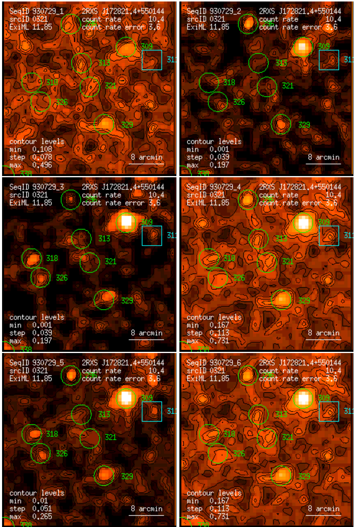
Figure 321: RASS 930729: detection 0321: band rate images, Gaussian filter: (1) PSPC channels 11 – 41, (2) 52 – 90, (3) 91 – 201, (4) 11 – 235, (5) 52 – 201, (6) 11 – 201. Broad band rates in counts/ks. Band rate contour levels in counts/ks/arcmin 2 .
