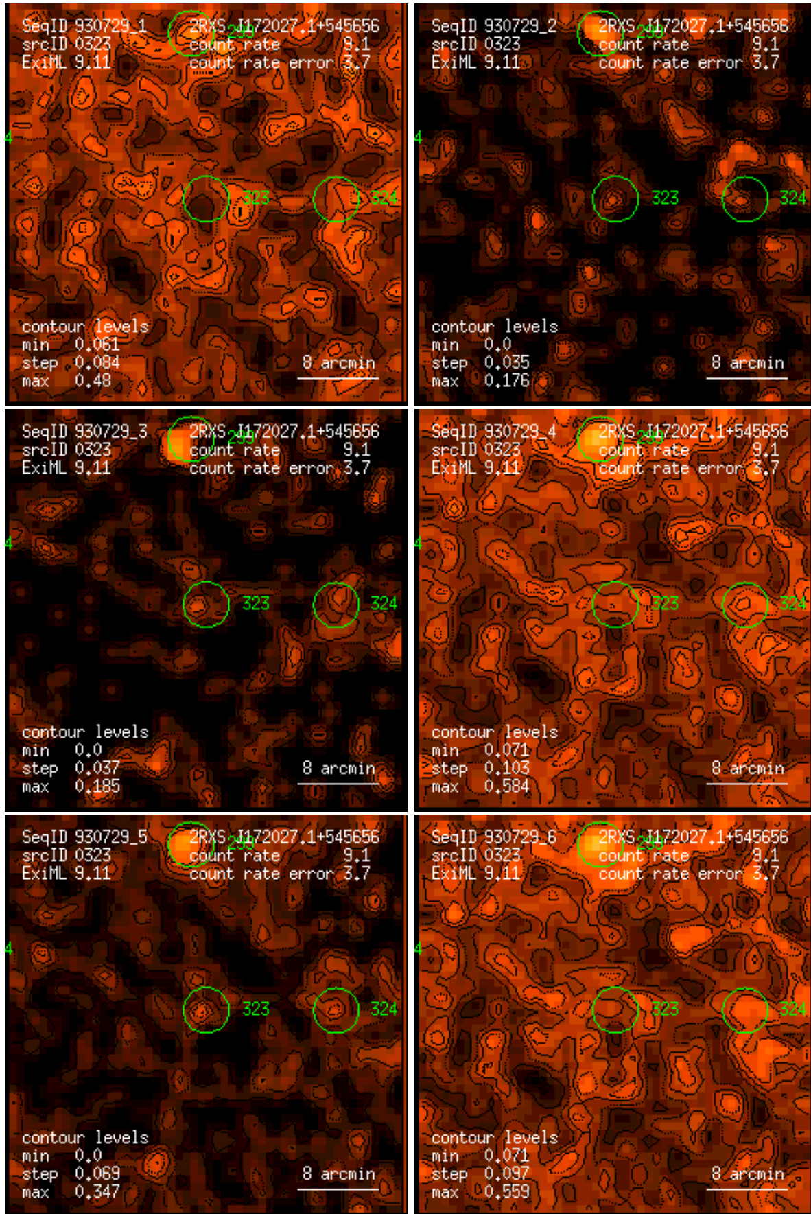
Figure 323: RASS 930729: detection 0323: band rate images, Gaussian filter: (1) PSPC channels 11 – 41, (2) 52 – 90, (3) 91 – 201, (4) 11 – 235, (5) 52 – 201, (6) 11 – 201. Broad band rates in counts/ks. Band rate contour levels in counts/ks/arcmin 2 .
