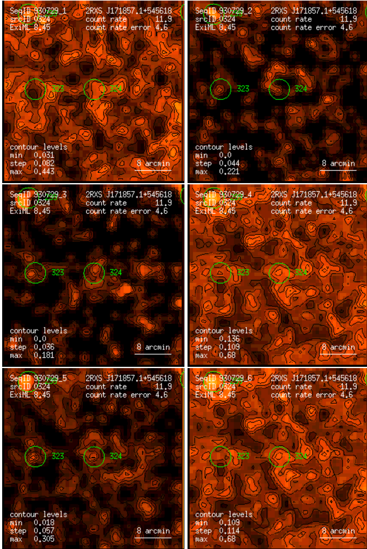
Figure 324: RASS 930729: detection 0324: band rate images, Gaussian filter: (1) PSPC channels 11 – 41, (2) 52 – 90, (3) 91 – 201, (4) 11 – 235, (5) 52 – 201, (6) 11 – 201. Broad band rates in counts/ks. Band rate contour levels in counts/ks/arcmin 2 .
