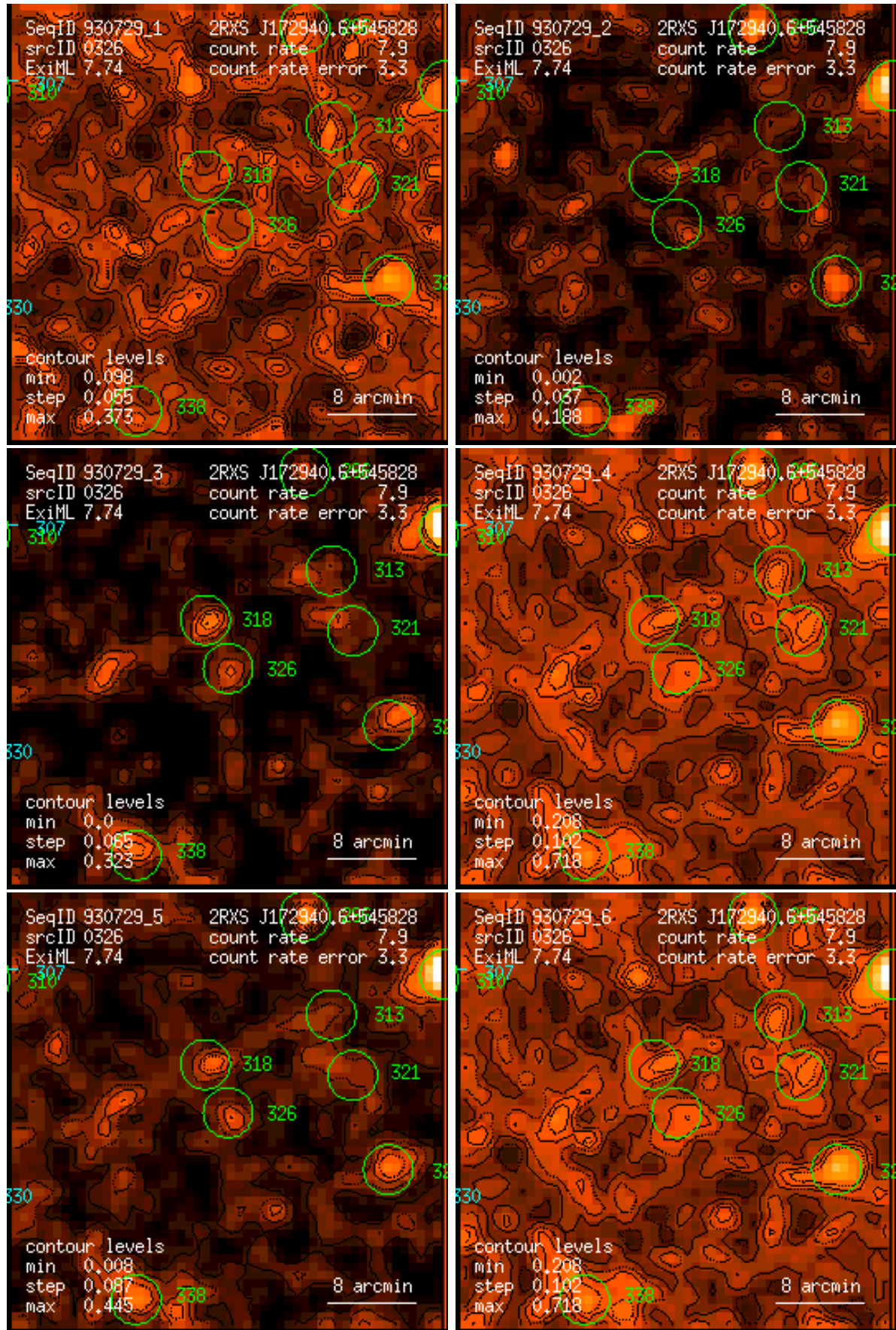
Figure 326: RASS 930729: detection 0326: band rate images, Gaussian filter: (1) PSPC channels 11 – 41, (2) 52 – 90, (3) 91 – 201, (4) 11 – 235, (5) 52 – 201, (6) 11 – 201. Broad band rates in counts/ks. Band rate contour levels in counts/ks/arcmin 2 .
