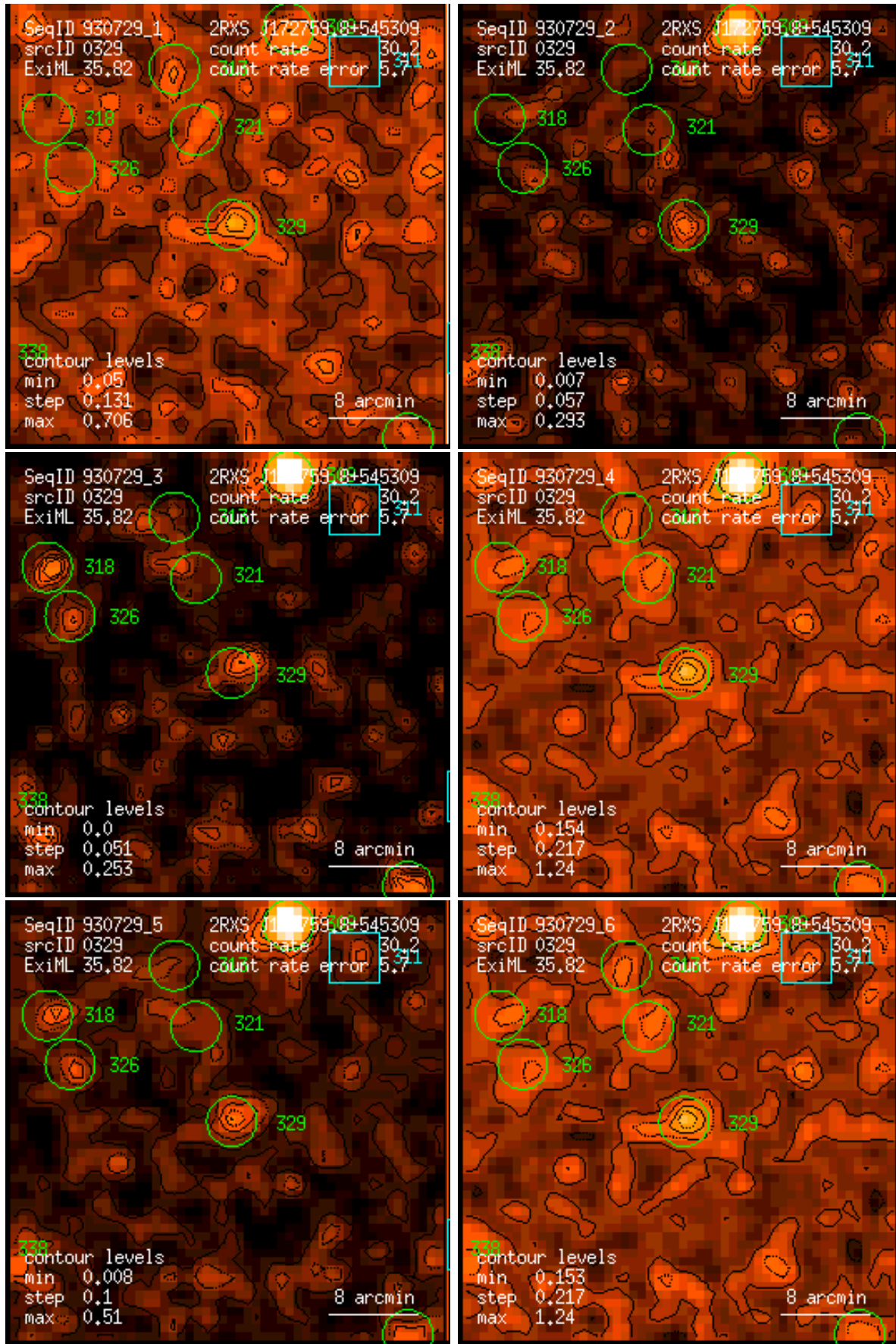
Figure 329: RASS 930729: detection 0329: band rate images, Gaussian filter: (1) PSPC channels 11 – 41, (2) 52 – 90, (3) 91 – 201, (4) 11 – 235, (5) 52 – 201, (6) 11 – 201. Broad band rates in counts/ks. Band rate contour levels in counts/ks/arcmin 2 .
