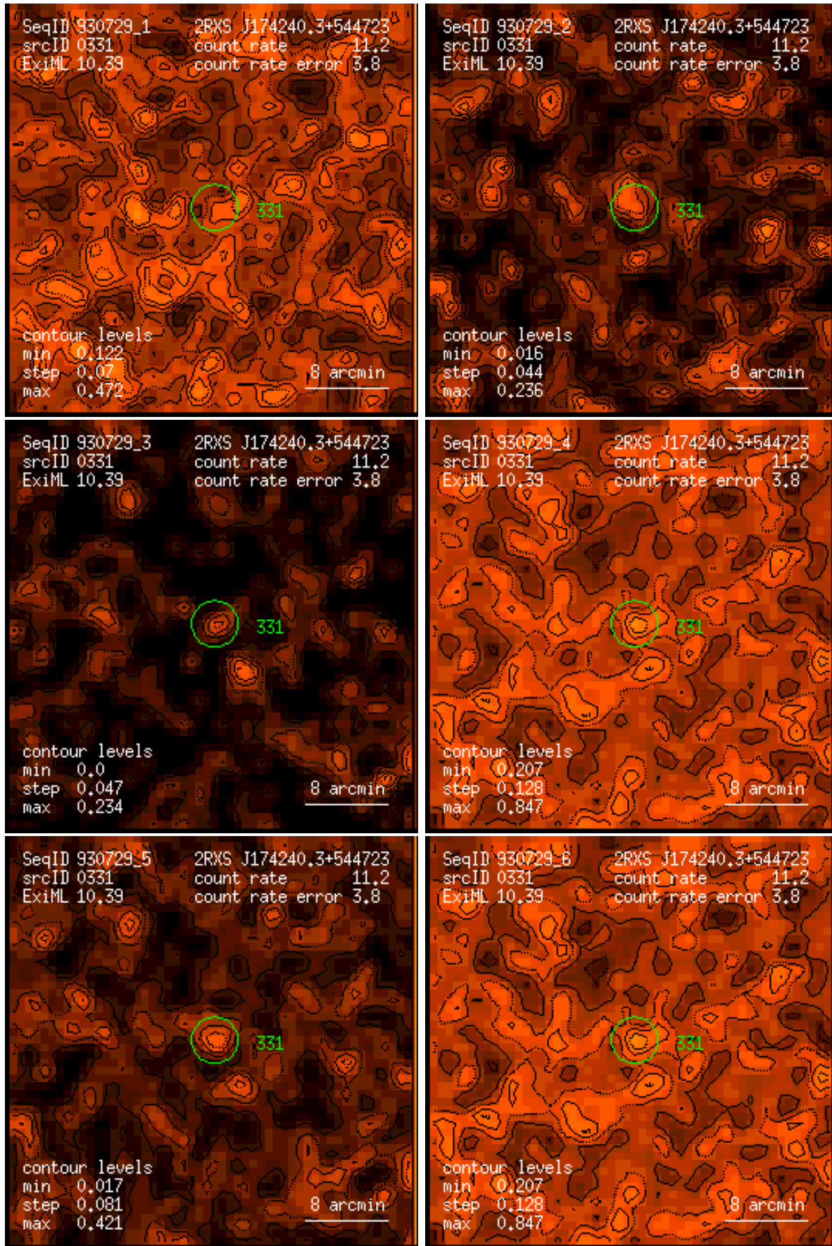
Figure 331: RASS 930729: detection 0331: band rate images, Gaussian filter: (1) PSPC channels 11 – 41, (2) 52 – 90, (3) 91 – 201, (4) 11 – 235, (5) 52 – 201, (6) 11 – 201. Broad band rates in counts/ks. Band rate contour levels in counts/ks/arcmin 2 .
