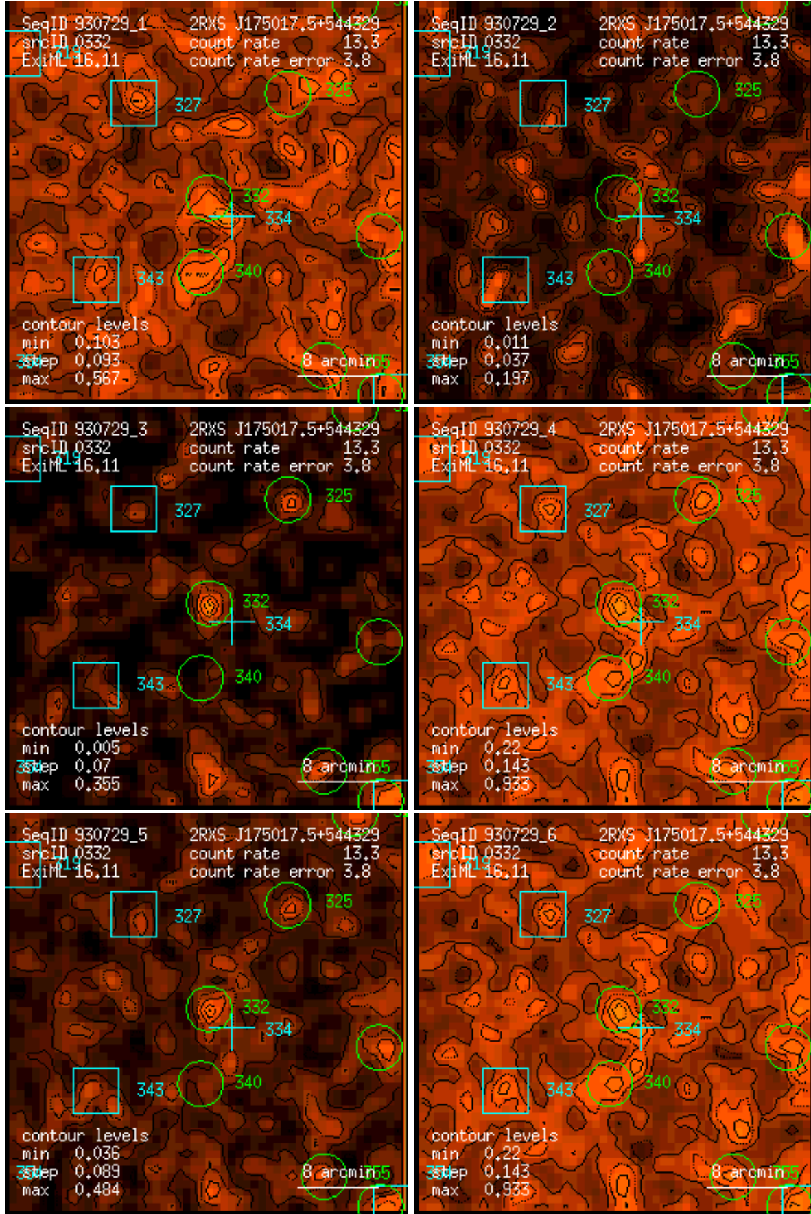
Figure 332: RASS 930729: detection 0332: band rate images, Gaussian filter: (1) PSPC channels 11 – 41, (2) 52 – 90, (3) 91 – 201, (4) 11 – 235, (5) 52 – 201, (6) 11 – 201. Broad band rates in counts/ks. Band rate contour levels in counts/ks/arcmin 2 .
