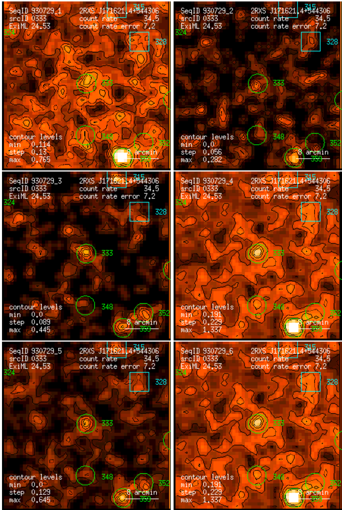
Figure 333: RASS 930729: detection 0333: band rate images, Gaussian filter: (1) PSPC channels 11 – 41, (2) 52 – 90, (3) 91 – 201, (4) 11 – 235, (5) 52 – 201, (6) 11 – 201. Broad band rates in counts/ks. Band rate contour levels in counts/ks/arcmin 2 .
