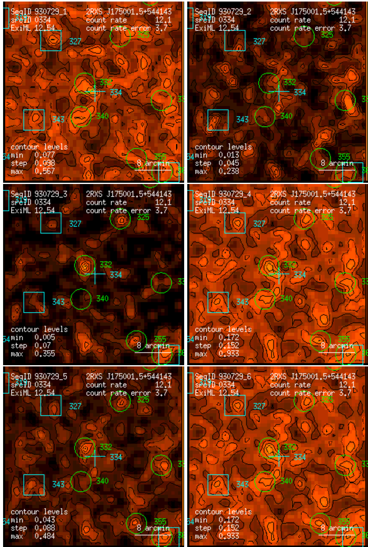
Figure 334: RASS 930729: detection 0334: band rate images, Gaussian filter: (1) PSPC channels 11 – 41, (2) 52 – 90, (3) 91 – 201, (4) 11 – 235, (5) 52 – 201, (6) 11 – 201. Broad band rates in counts/ks. Band rate contour levels in counts/ks/arcmin 2 .
