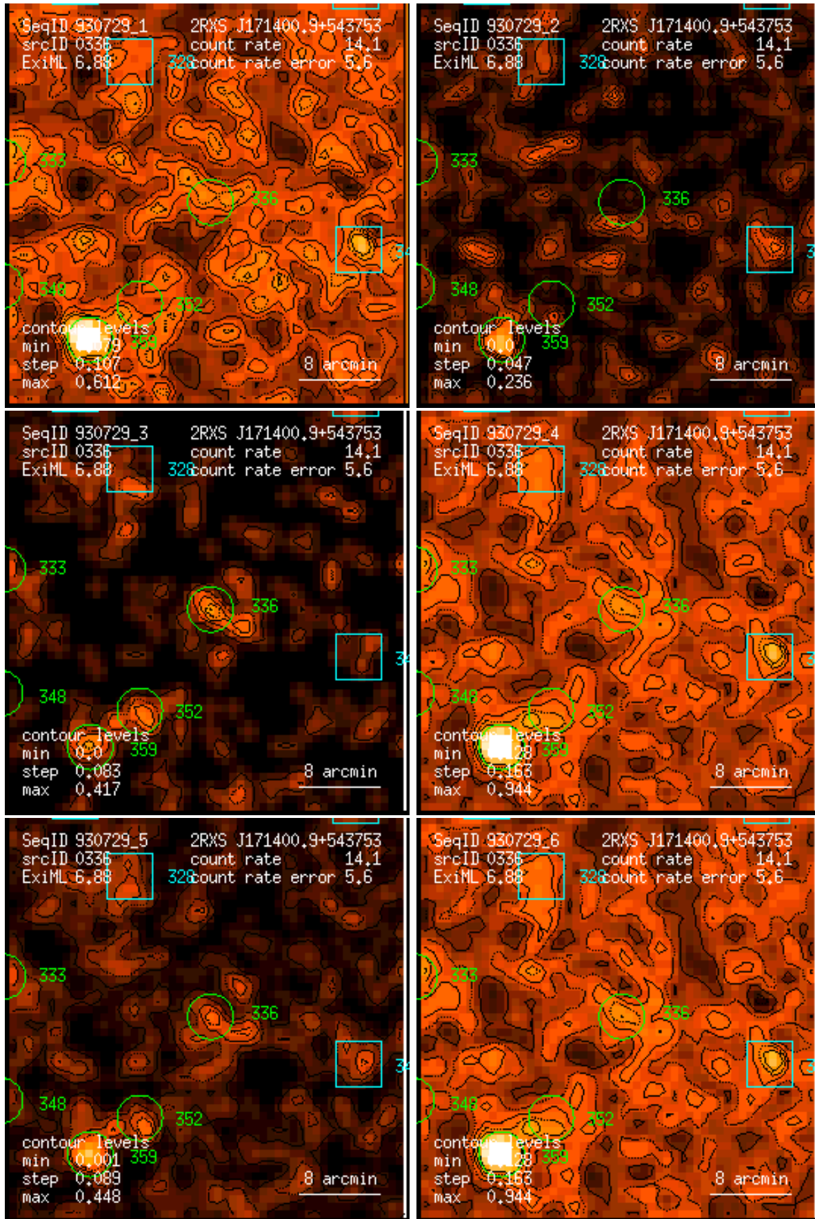
Figure 336: RASS 930729: detection 0336: band rate images, Gaussian filter: (1) PSPC channels 11 – 41, (2) 52 – 90, (3) 91 – 201, (4) 11 – 235, (5) 52 – 201, (6) 11 – 201. Broad band rates in counts/ks. Band rate contour levels in counts/ks/arcmin 2 .
