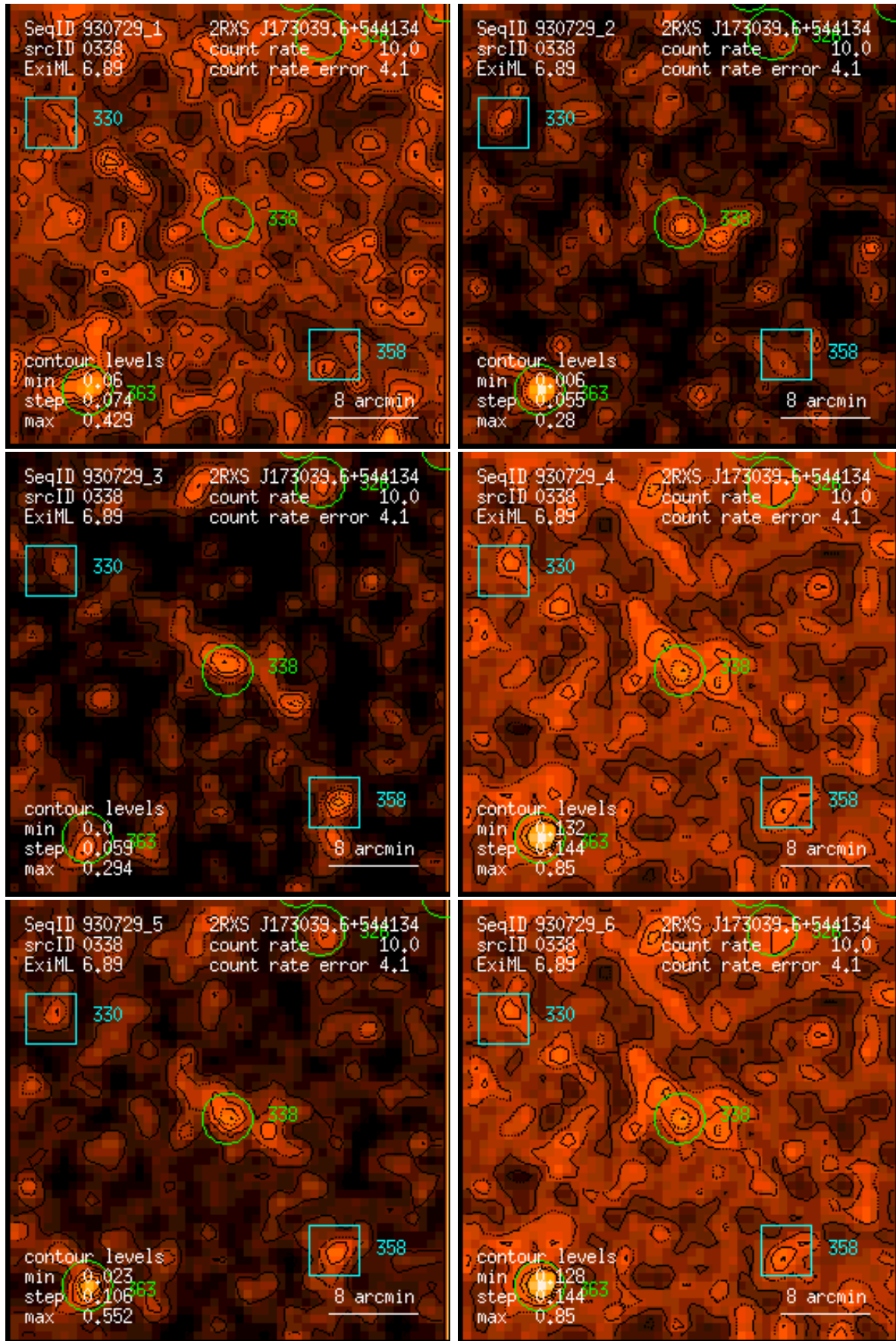
Figure 338: RASS 930729: detection 0338: band rate images, Gaussian filter: (1) PSPC channels 11 – 41, (2) 52 – 90, (3) 91 – 201, (4) 11 – 235, (5) 52 – 201, (6) 11 – 201. Broad band rates in counts/ks. Band rate contour levels in counts/ks/arcmin 2 .
