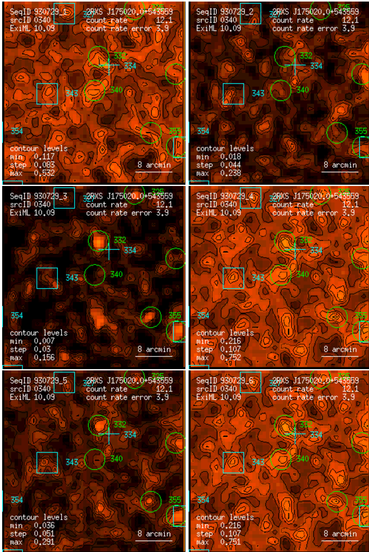
Figure 340: RASS 930729: detection 0340: band rate images, Gaussian filter: (1) PSPC channels 11 – 41, (2) 52 – 90, (3) 91 – 201, (4) 11 – 235, (5) 52 – 201, (6) 11 – 201. Broad band rates in counts/ks. Band rate contour levels in counts/ks/arcmin 2 .
