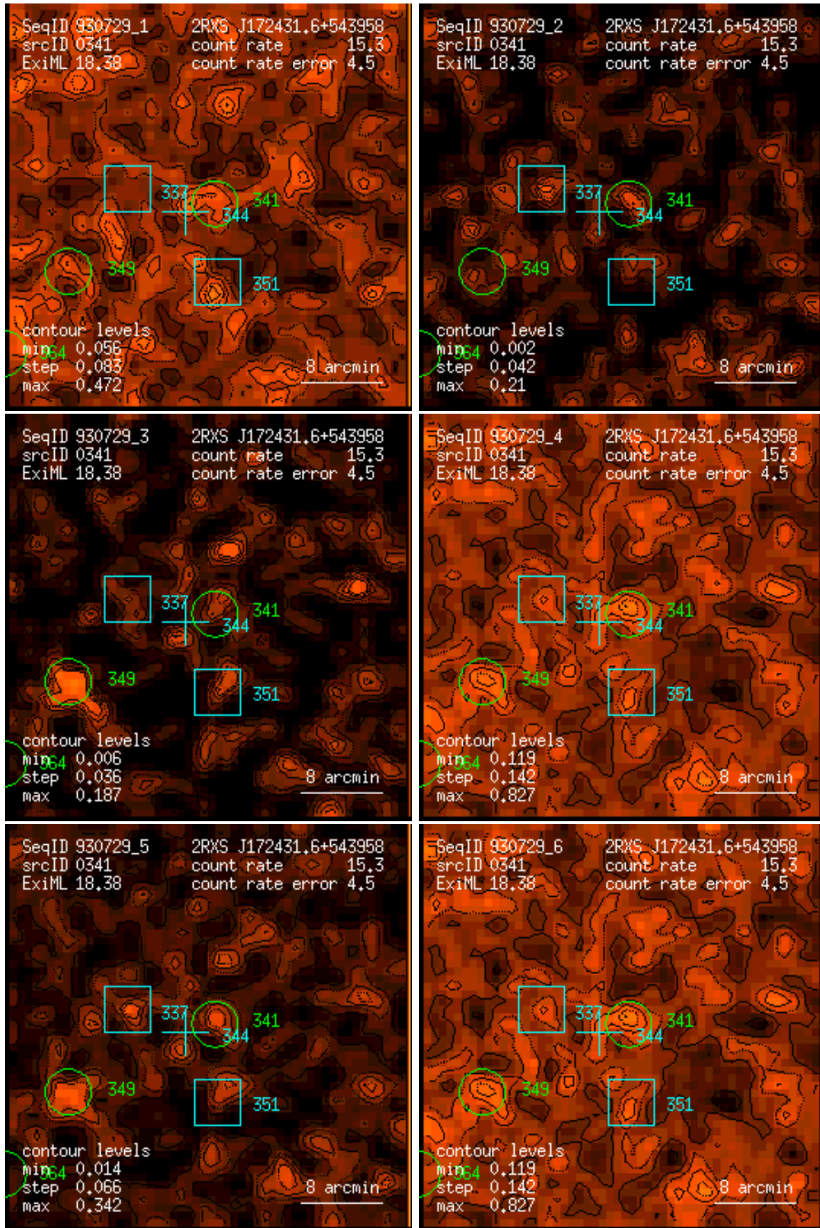
Figure 341: RASS 930729: detection 0341: band rate images, Gaussian filter: (1) PSPC channels 11 – 41, (2) 52 – 90, (3) 91 – 201, (4) 11 – 235, (5) 52 – 201, (6) 11 – 201. Broad band rates in counts/ks. Band rate contour levels in counts/ks/arcmin 2 .
