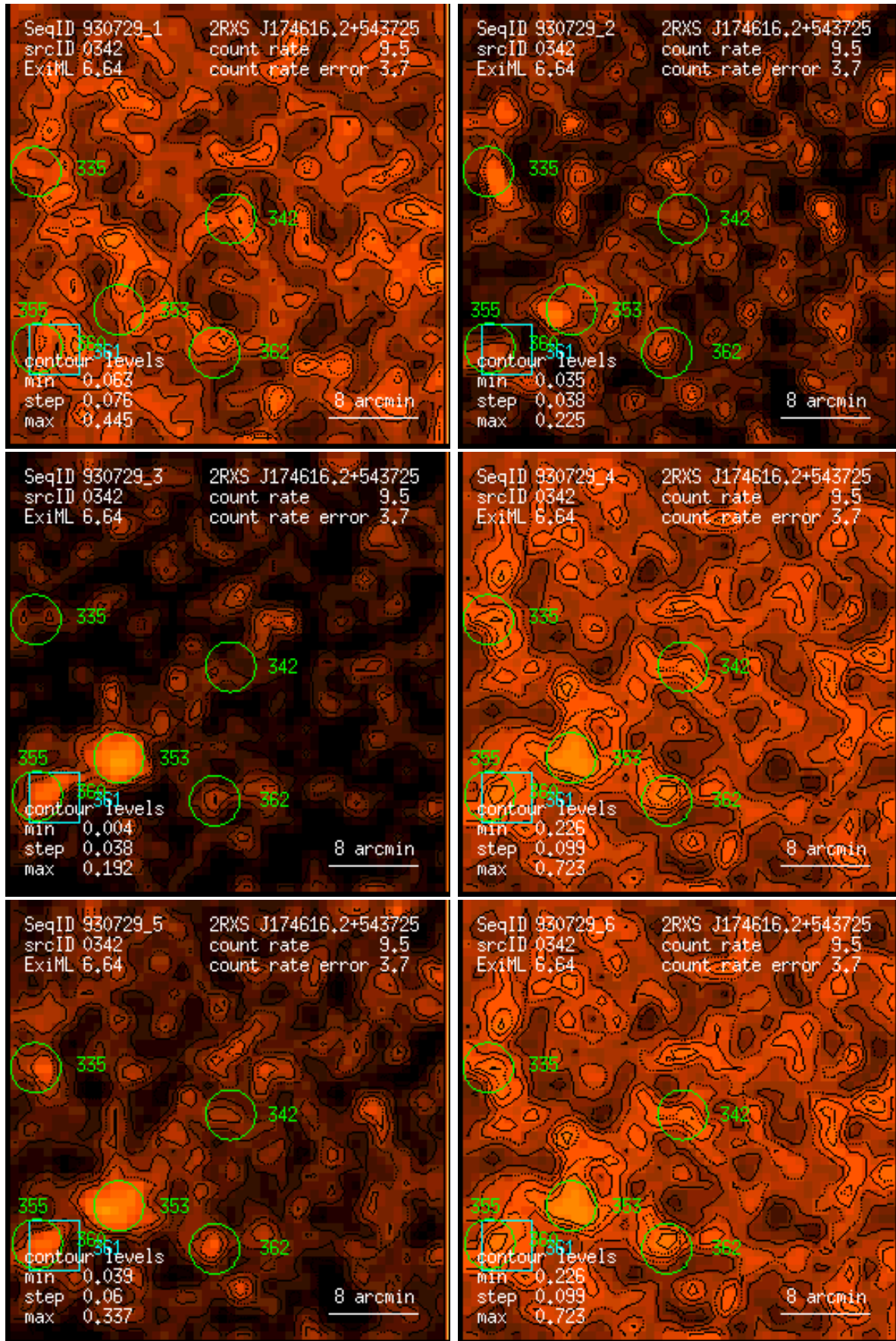
Figure 342: RASS 930729: detection 0342: band rate images, Gaussian filter: (1) PSPC channels 11 – 41, (2) 52 – 90, (3) 91 – 201, (4) 11 – 235, (5) 52 – 201, (6) 11 – 201. Broad band rates in counts/ks. Band rate contour levels in counts/ks/arcmin 2 .
