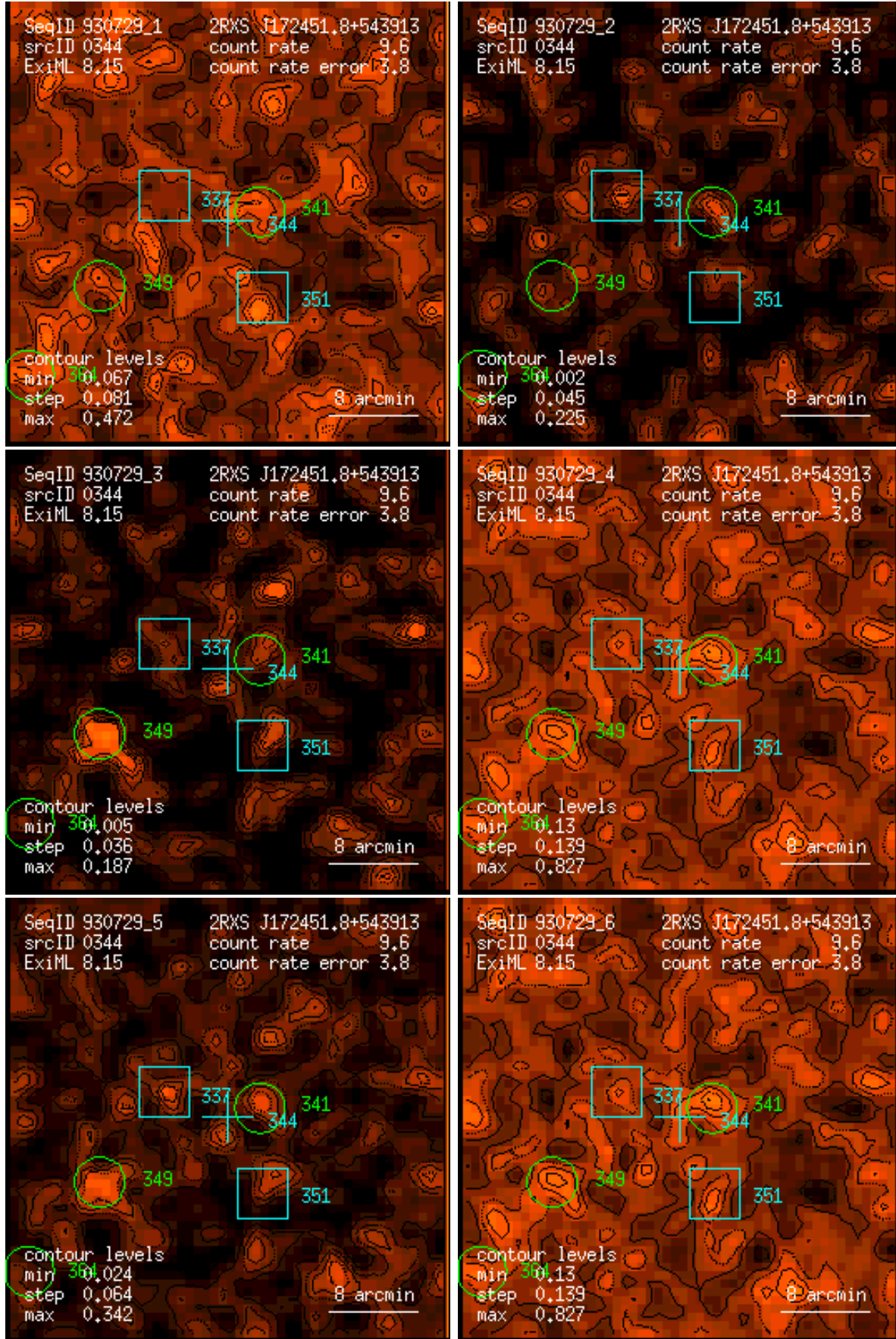
Figure 344: RASS 930729: detection 0344: band rate images, Gaussian filter: (1) PSPC channels 11 – 41, (2) 52 – 90, (3) 91 – 201, (4) 11 – 235, (5) 52 – 201, (6) 11 – 201. Broad band rates in counts/ks. Band rate contour levels in counts/ks/arcmin 2 .
