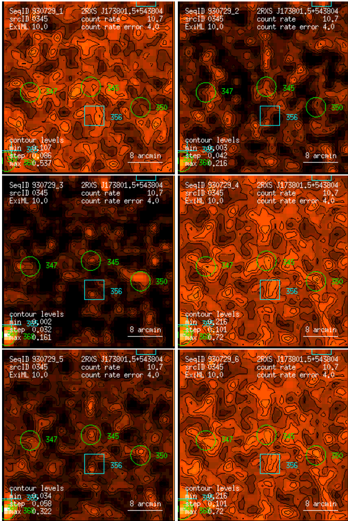
Figure 345: RASS 930729: detection 0345: band rate images, Gaussian filter: (1) PSPC channels 11 – 41, (2) 52 – 90, (3) 91 – 201, (4) 11 – 235, (5) 52 – 201, (6) 11 – 201. Broad band rates in counts/ks. Band rate contour levels in counts/ks/arcmin 2 .
