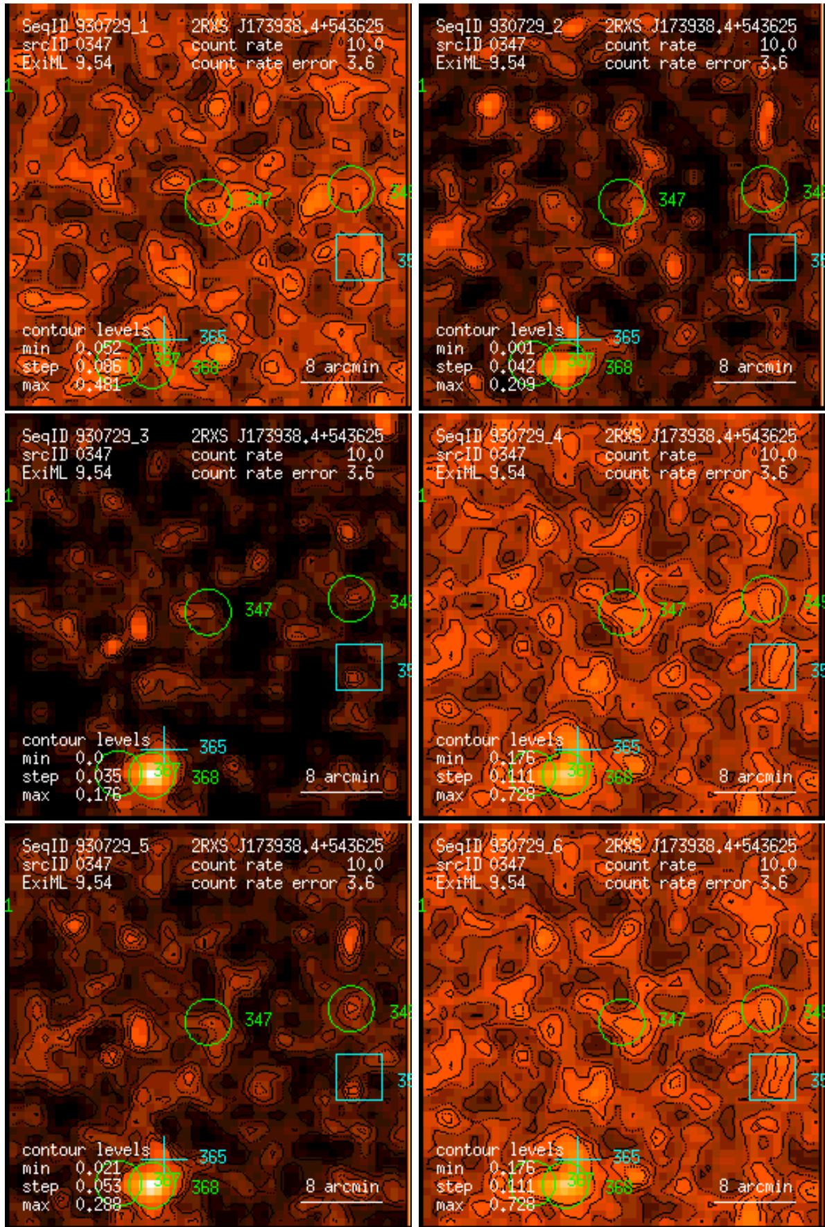
Figure 347: RASS 930729: detection 0347: band rate images, Gaussian filter: (1) PSPC channels 11 – 41, (2) 52 – 90, (3) 91 – 201, (4) 11 – 235, (5) 52 – 201, (6) 11 – 201. Broad band rates in counts/ks. Band rate contour levels in counts/ks/arcmin 2 .
