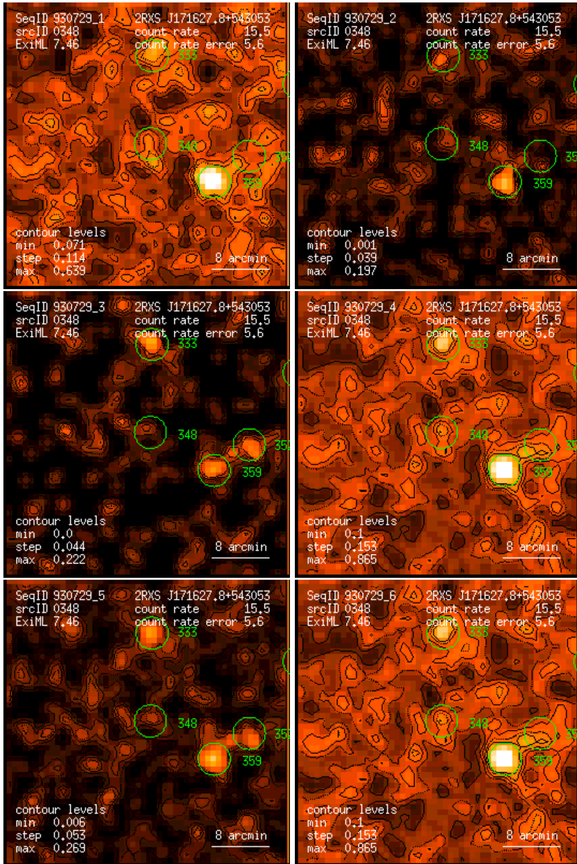
Figure 348: RASS 930729: detection 0348: band rate images, Gaussian filter: (1) PSPC channels 11 – 41, (2) 52 – 90, (3) 91 – 201, (4) 11 – 235, (5) 52 – 201, (6) 11 – 201. Broad band rates in counts/ks. Band rate contour levels in counts/ks/arcmin 2 .
