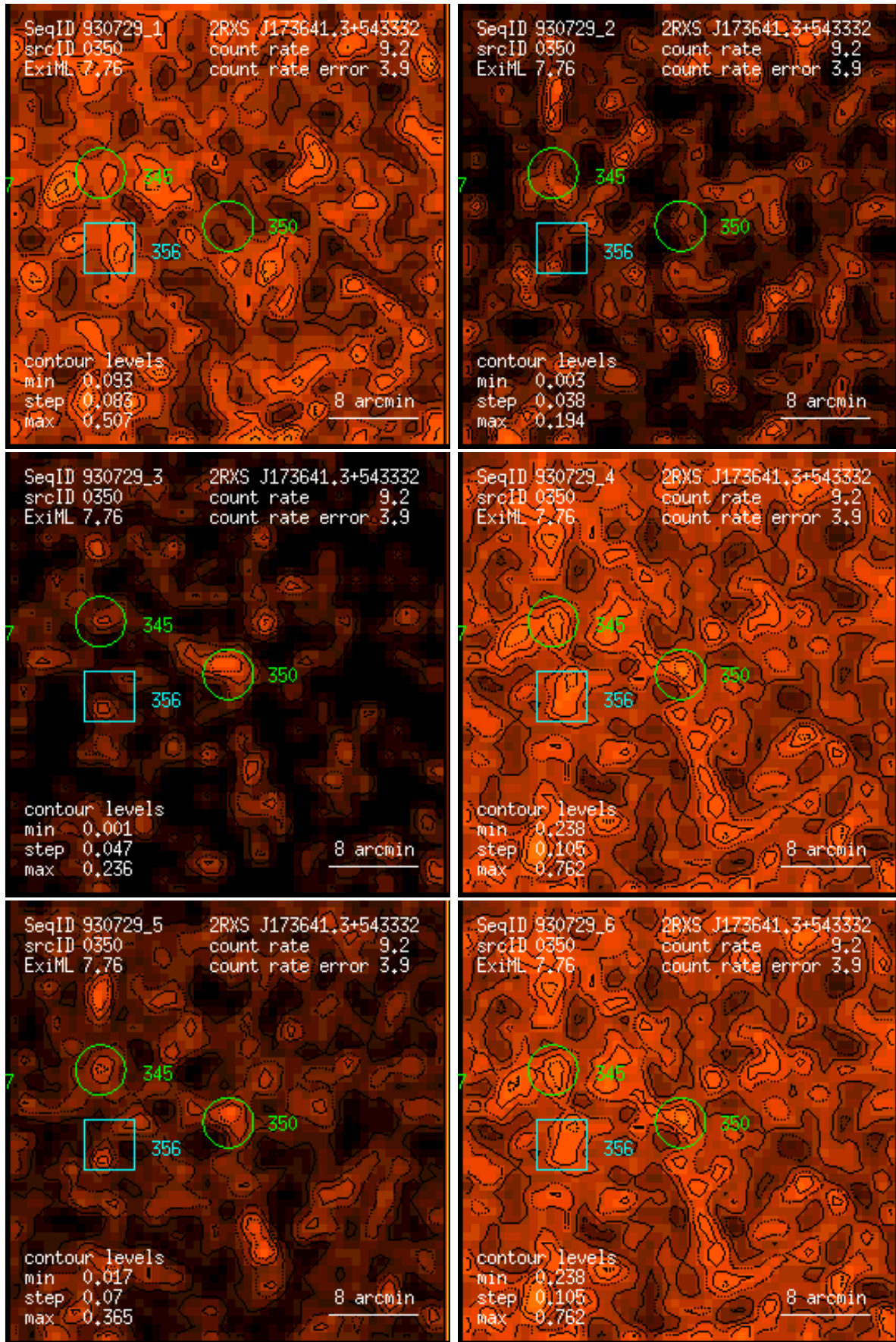
Figure 350: RASS 930729: detection 0350: band rate images, Gaussian filter: (1) PSPC channels 11 – 41, (2) 52 – 90, (3) 91 – 201, (4) 11 – 235, (5) 52 – 201, (6) 11 – 201. Broad band rates in counts/ks. Band rate contour levels in counts/ks/arcmin 2 .
