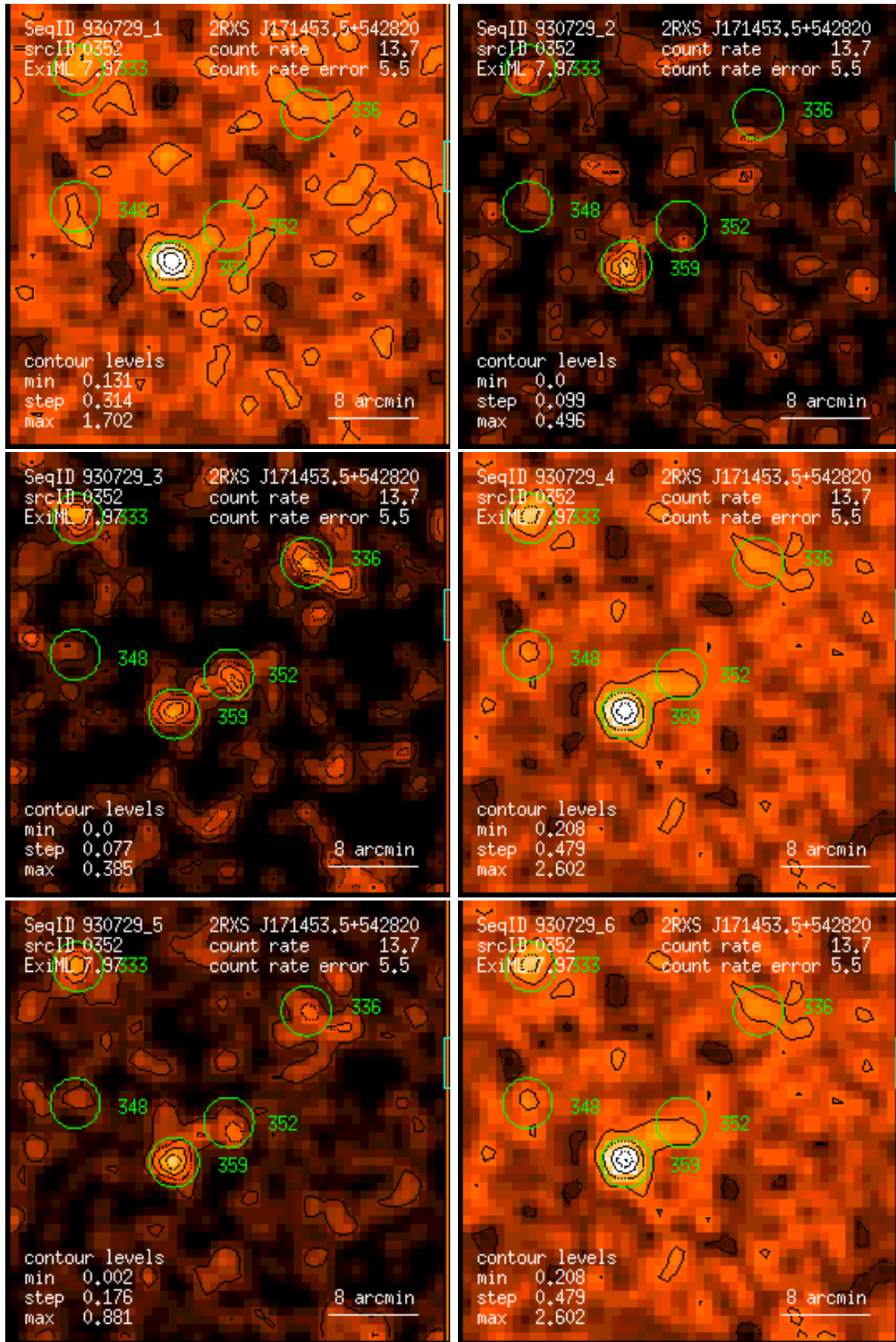
Figure 352: RASS 930729: detection 0352: band rate images, Gaussian filter: (1) PSPC channels 11 – 41, (2) 52 – 90, (3) 91 – 201, (4) 11 – 235, (5) 52 – 201, (6) 11 – 201. Broad band rates in counts/ks. Band rate contour levels in counts/ks/arcmin 2 .
