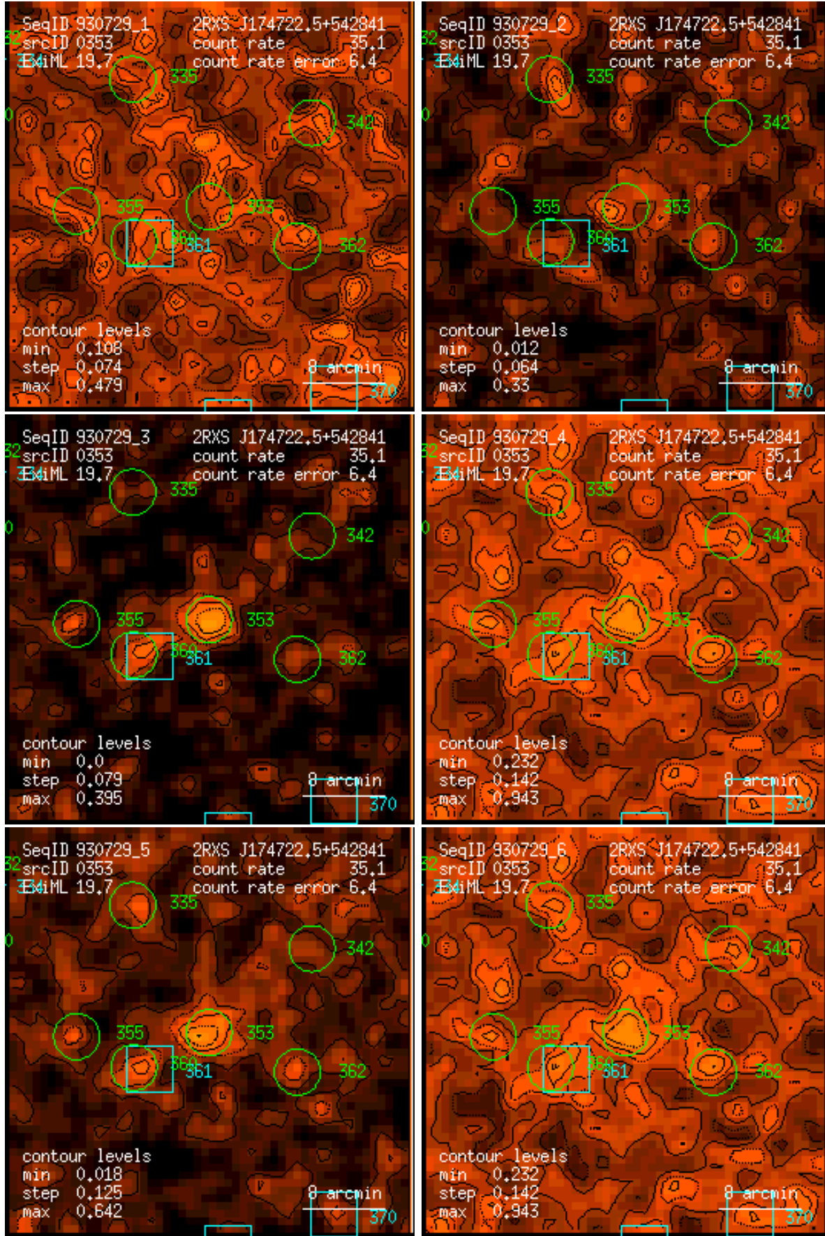
Figure 353: RASS 930729: detection 0353: band rate images, Gaussian filter: (1) PSPC channels 11 – 41, (2) 52 – 90, (3) 91 – 201, (4) 11 – 235, (5) 52 – 201, (6) 11 – 201. Broad band rates in counts/ks. Band rate contour levels in counts/ks/arcmin 2 .
