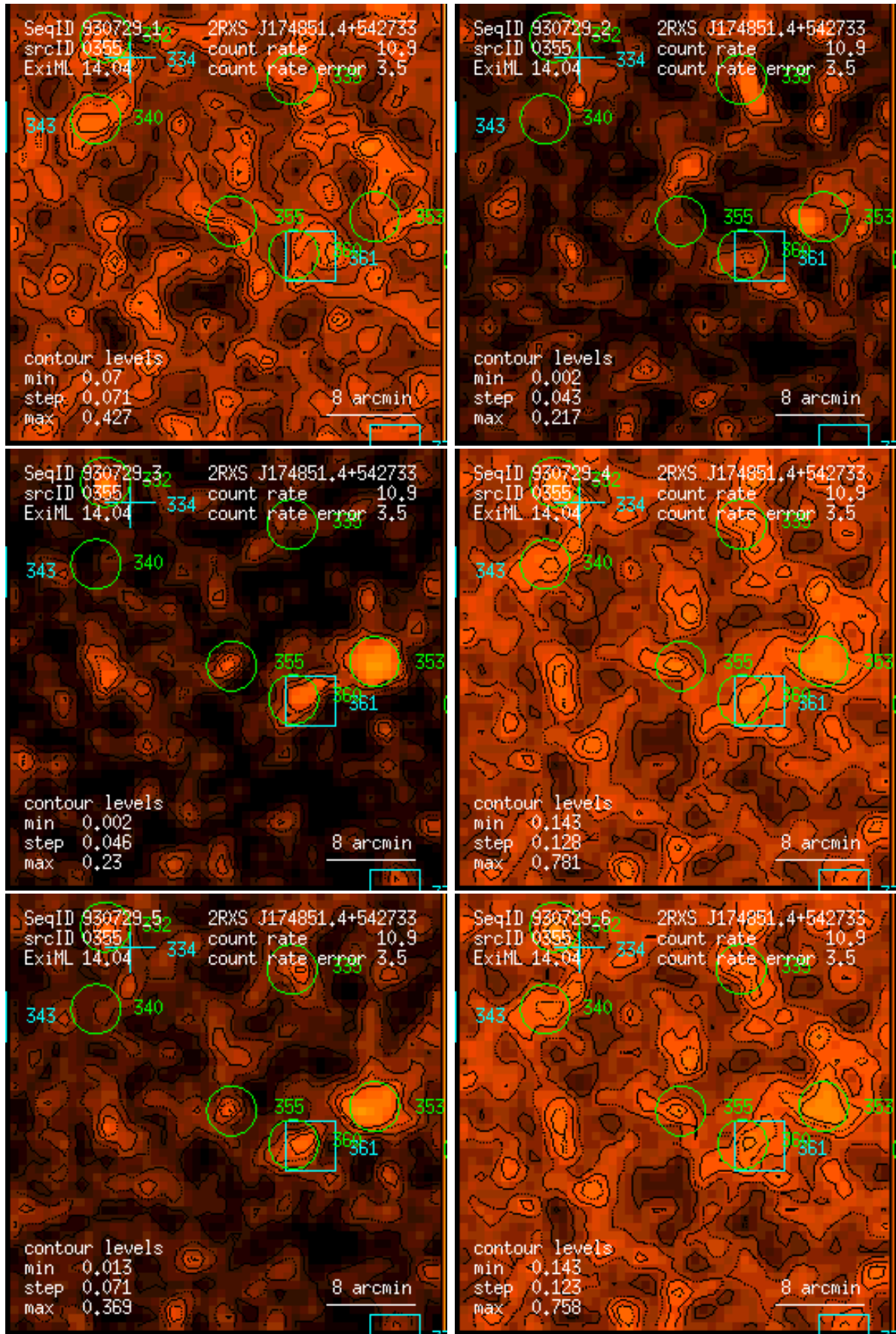
Figure 355: RASS 930729: detection 0355: band rate images, Gaussian filter: (1) PSPC channels 11 – 41, (2) 52 – 90, (3) 91 – 201, (4) 11 – 235, (5) 52 – 201, (6) 11 – 201. Broad band rates in counts/ks. Band rate contour levels in counts/ks/arcmin 2 .
