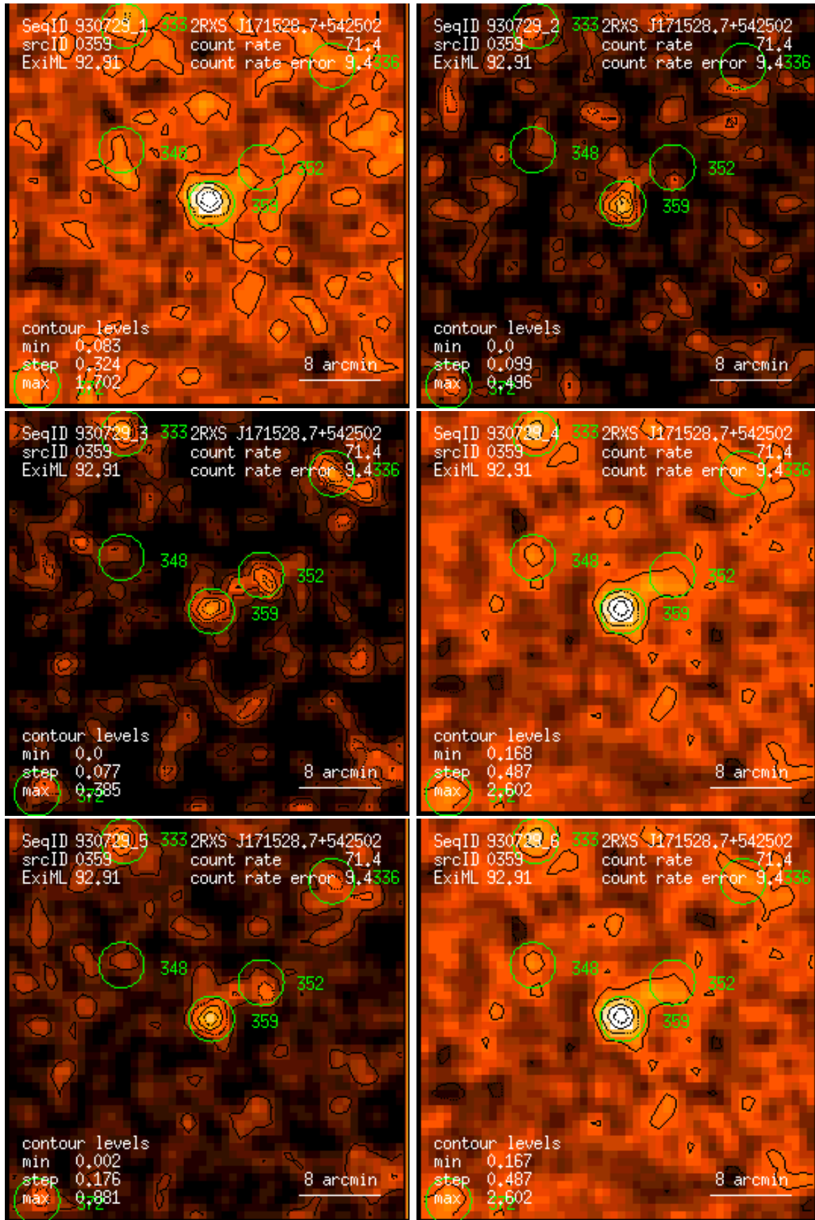
Figure 359: RASS 930729: detection 0359: band rate images, Gaussian filter: (1) PSPC channels 11 – 41, (2) 52 – 90, (3) 91 – 201, (4) 11 – 235, (5) 52 – 201, (6) 11 – 201. Broad band rates in counts/ks. Band rate contour levels in counts/ks/arcmin 2 .
