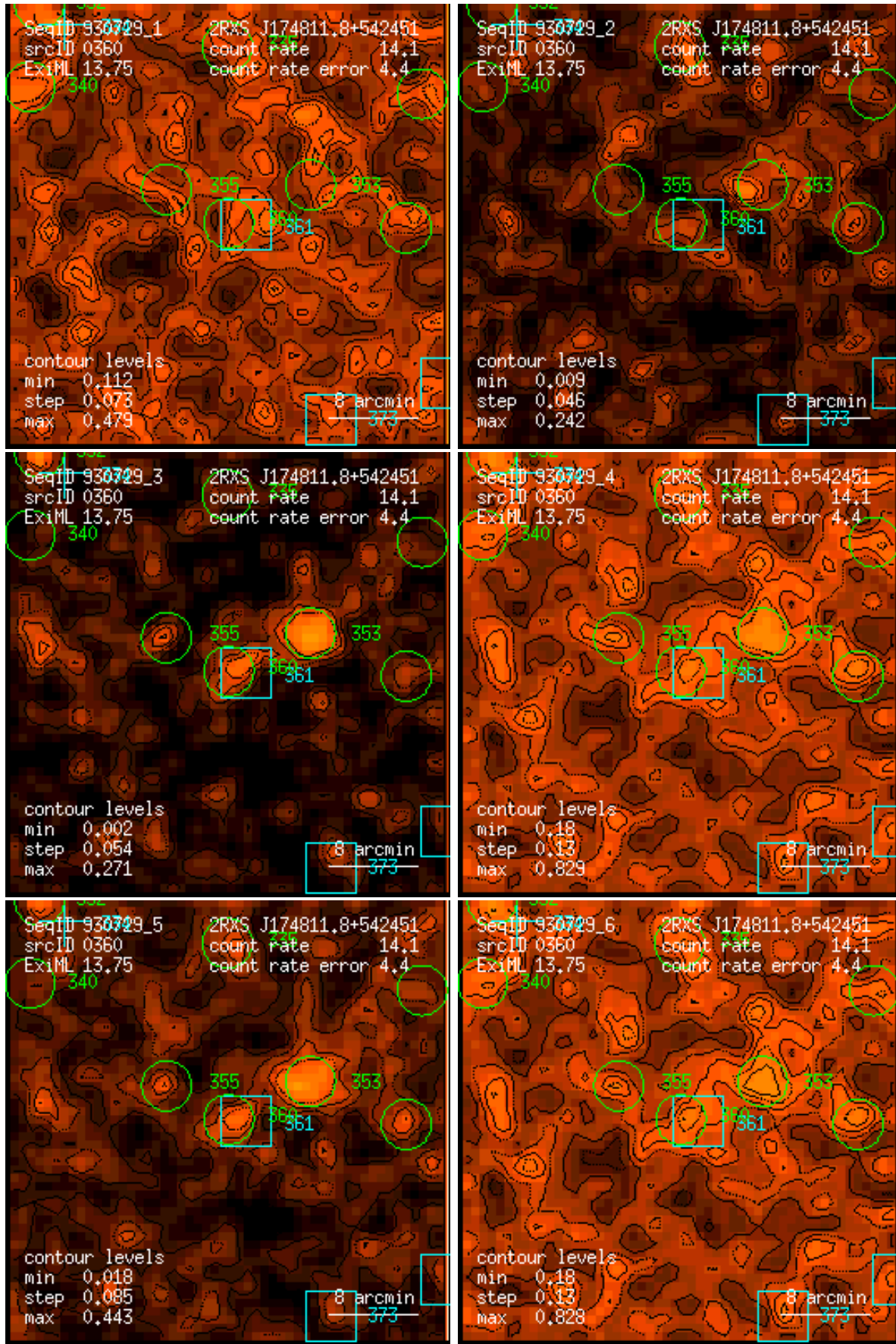
Figure 360: RASS 930729: detection 0360: band rate images, Gaussian filter: (1) PSPC channels 11 – 41, (2) 52 – 90, (3) 91 – 201, (4) 11 – 235, (5) 52 – 201, (6) 11 – 201. Broad band rates in counts/ks. Band rate contour levels in counts/ks/arcmin 2 .
