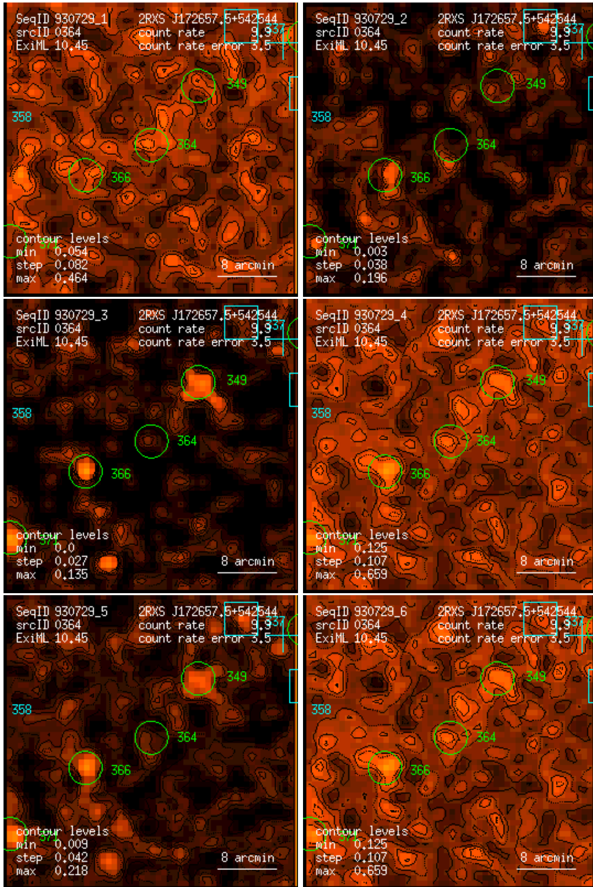
Figure 364: RASS 930729: detection 0364: band rate images, Gaussian filter: (1) PSPC channels 11 – 41, (2) 52 – 90, (3) 91 – 201, (4) 11 – 235, (5) 52 – 201, (6) 11 – 201. Broad band rates in counts/ks. Band rate contour levels in counts/ks/arcmin 2 .
