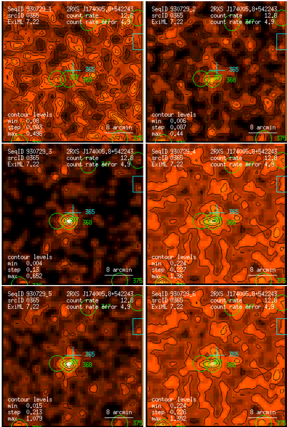
Figure 365: RASS 930729: detection 0365: band rate images, Gaussian filter: (1) PSPC channels 11 – 41, (2) 52 – 90, (3) 91 – 201, (4) 11 – 235, (5) 52 – 201, (6) 11 – 201. Broad band rates in counts/ks. Band rate contour levels in counts/ks/arcmin 2 .
