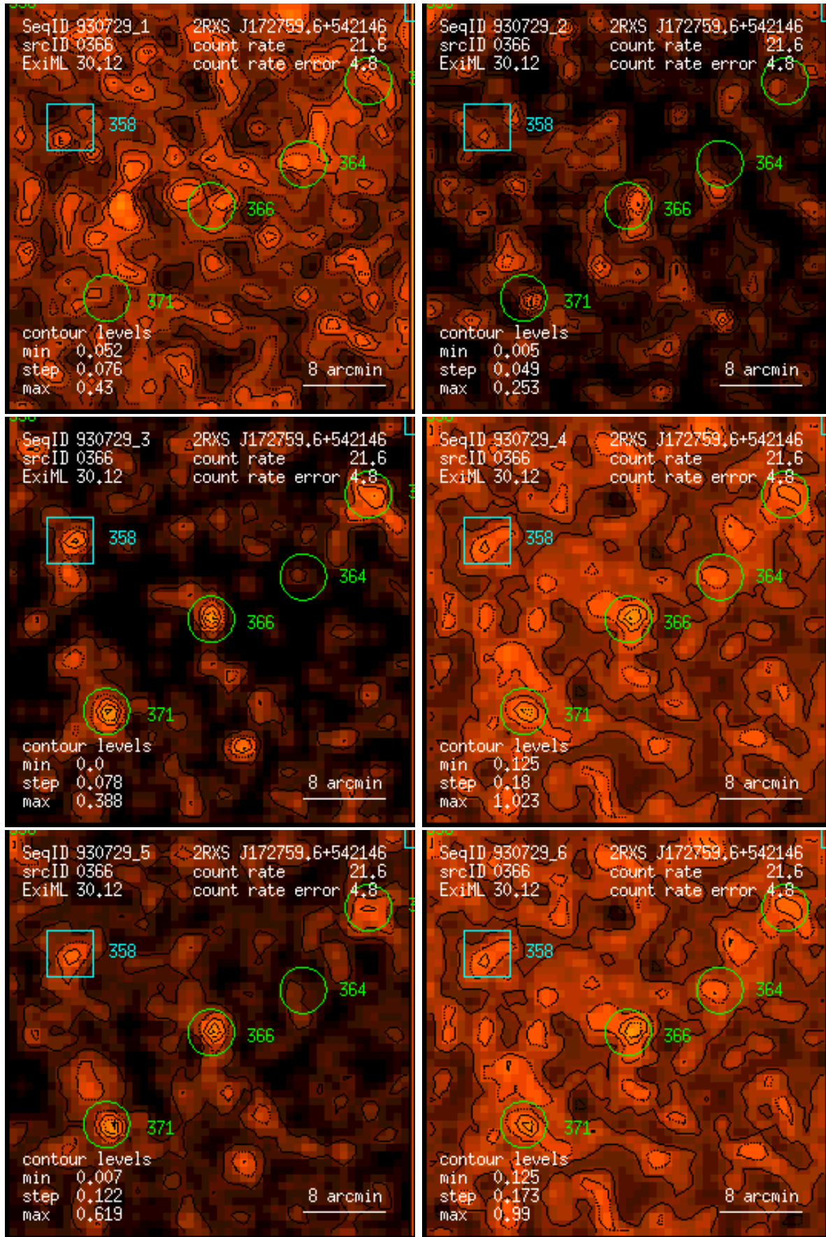
Figure 366: RASS 930729: detection 0366: band rate images, Gaussian filter: (1) PSPC channels 11 – 41, (2) 52 – 90, (3) 91 – 201, (4) 11 – 235, (5) 52 – 201, (6) 11 – 201. Broad band rates in counts/ks. Band rate contour levels in counts/ks/arcmin 2 .
