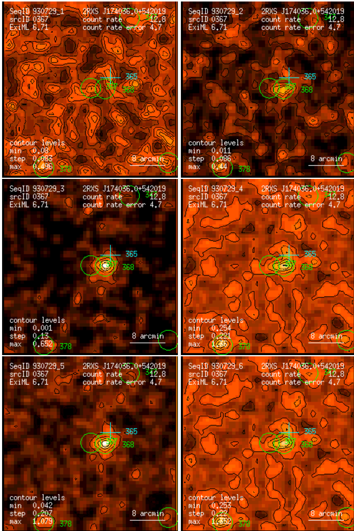
Figure 367: RASS 930729: detection 0367: band rate images, Gaussian filter: (1) PSPC channels 11 – 41, (2) 52 – 90, (3) 91 – 201, (4) 11 – 235, (5) 52 – 201, (6) 11 – 201. Broad band rates in counts/ks. Band rate contour levels in counts/ks/arcmin 2 .
