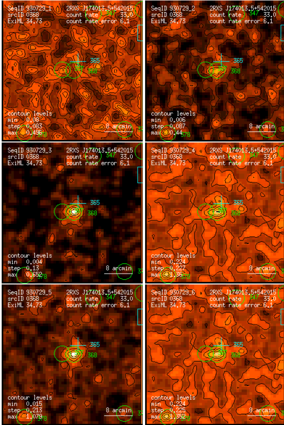
Figure 368: RASS 930729: detection 0368: band rate images, Gaussian filter: (1) PSPC channels 11 – 41, (2) 52 – 90, (3) 91 – 201, (4) 11 – 235, (5) 52 – 201, (6) 11 – 201. Broad band rates in counts/ks. Band rate contour levels in counts/ks/arcmin 2 .
