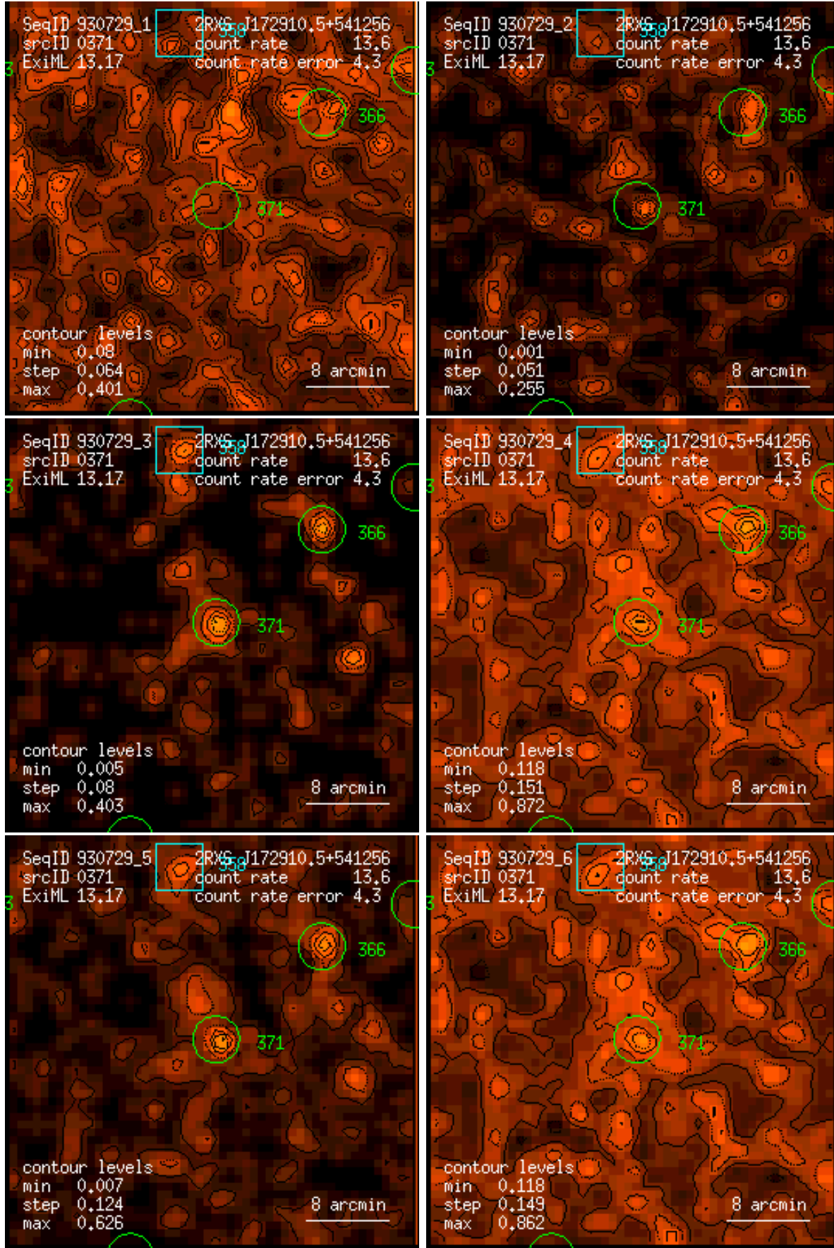
Figure 371: RASS 930729: detection 0371: band rate images, Gaussian filter: (1) PSPC channels 11 – 41, (2) 52 – 90, (3) 91 – 201, (4) 11 – 235, (5) 52 – 201, (6) 11 – 201. Broad band rates in counts/ks. Band rate contour levels in counts/ks/arcmin 2 .
