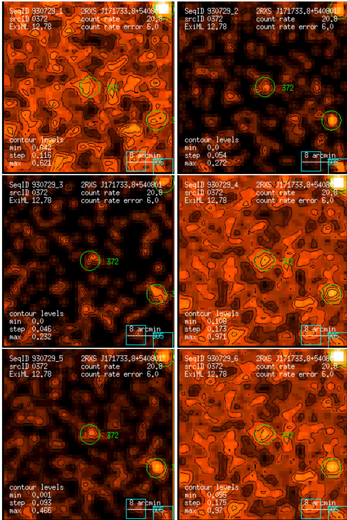
Figure 372: RASS 930729: detection 0372: band rate images, Gaussian filter: (1) PSPC channels 11 – 41, (2) 52 – 90, (3) 91 – 201, (4) 11 – 235, (5) 52 – 201, (6) 11 – 201. Broad band rates in counts/ks. Band rate contour levels in counts/ks/arcmin 2 .
