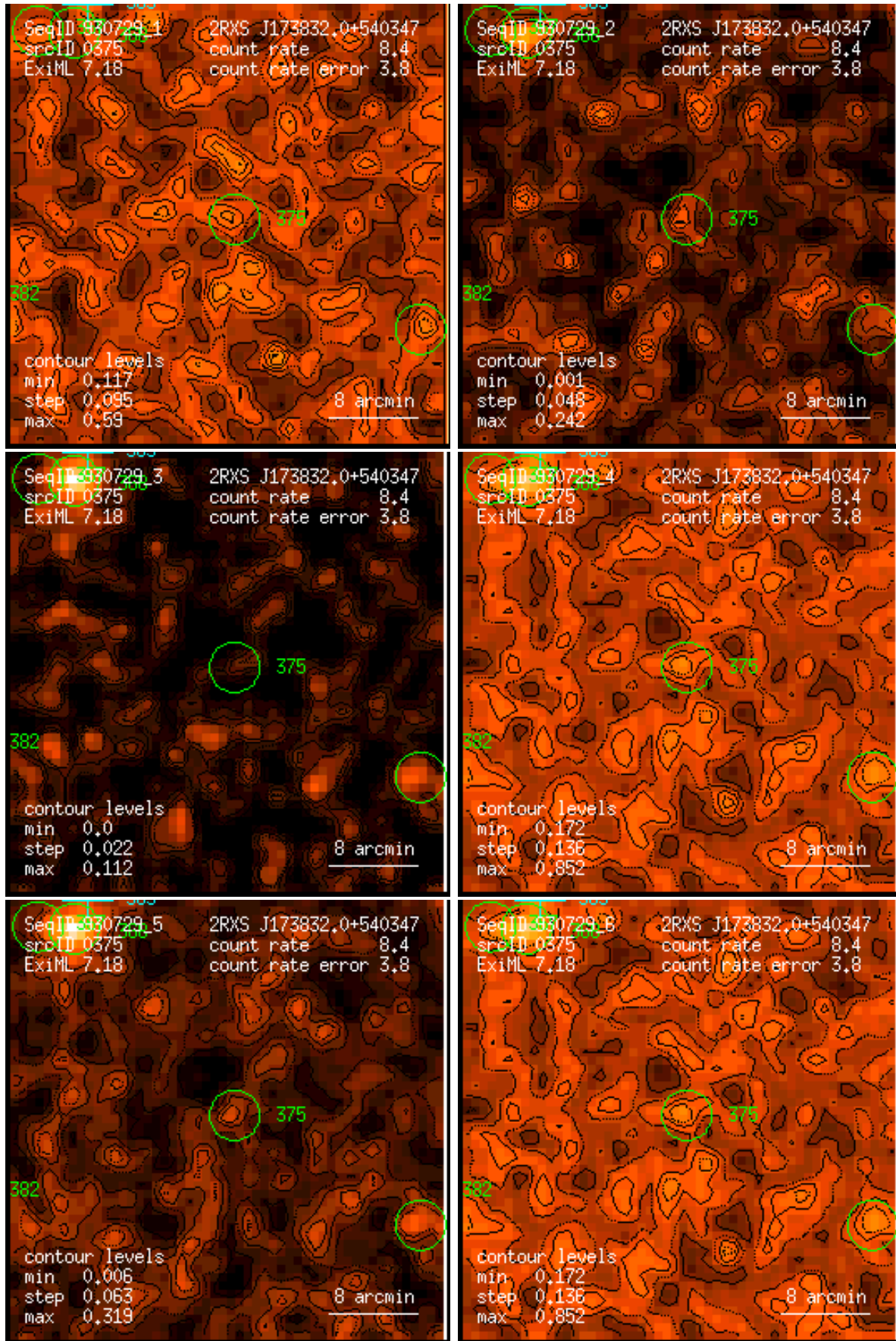
Figure 375: RASS 930729: detection 0375: band rate images, Gaussian filter: (1) PSPC channels 11 – 41, (2) 52 – 90, (3) 91 – 201, (4) 11 – 235, (5) 52 – 201, (6) 11 – 201. Broad band rates in counts/ks. Band rate contour levels in counts/ks/arcmin 2 .
