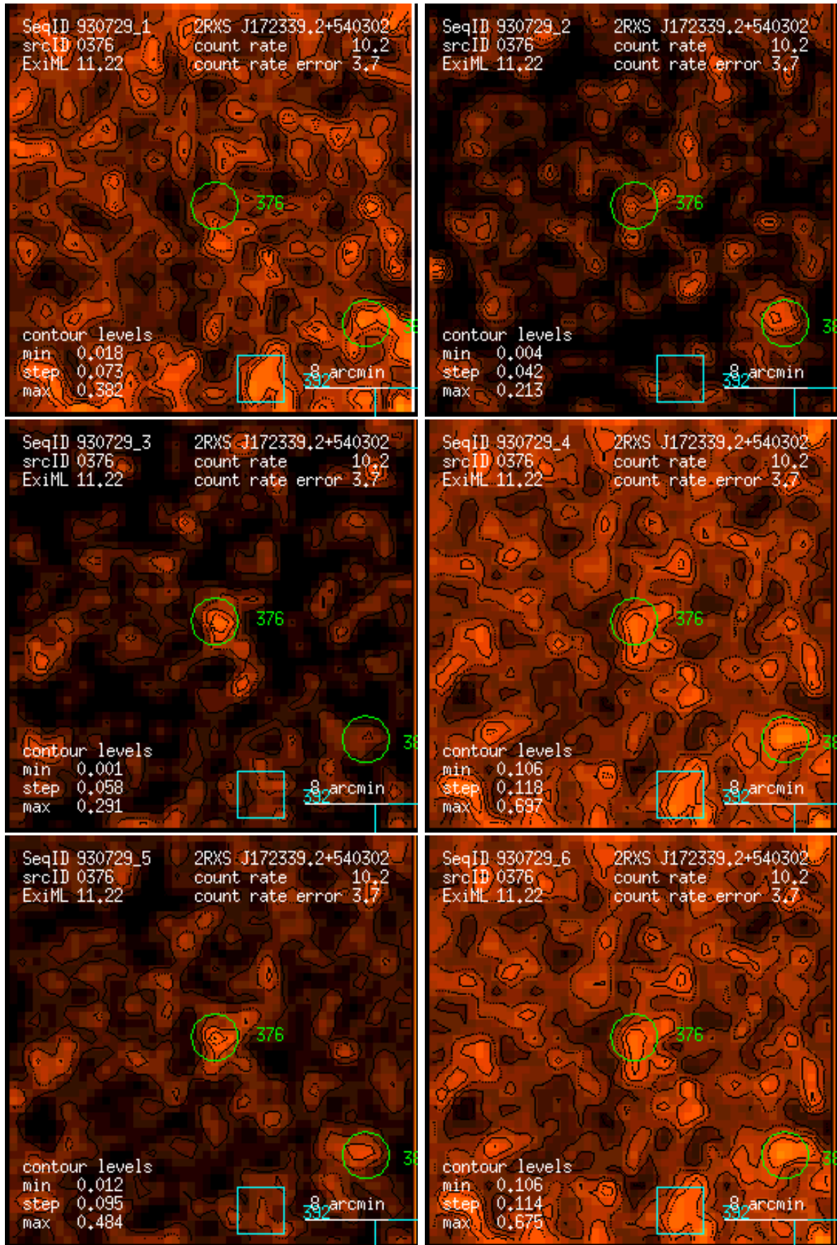
Figure 376: RASS 930729: detection 0376: band rate images, Gaussian filter: (1) PSPC channels 11 – 41, (2) 52 – 90, (3) 91 – 201, (4) 11 – 235, (5) 52 – 201, (6) 11 – 201. Broad band rates in counts/ks. Band rate contour levels in counts/ks/arcmin 2 .
