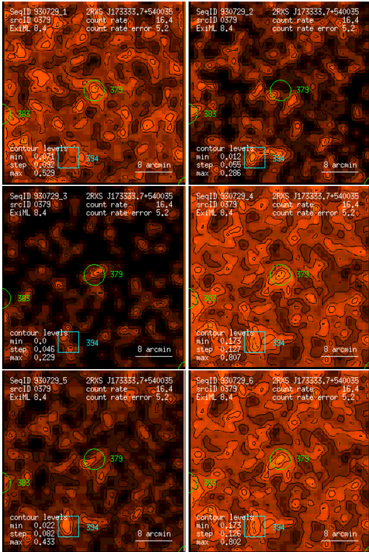
Figure 379: RASS 930729: detection 0379: band rate images, Gaussian filter: (1) PSPC channels 11 – 41, (2) 52 – 90, (3) 91 – 201, (4) 11 – 235, (5) 52 – 201, (6) 11 – 201. Broad band rates in counts/ks. Band rate contour levels in counts/ks/arcmin 2 .
