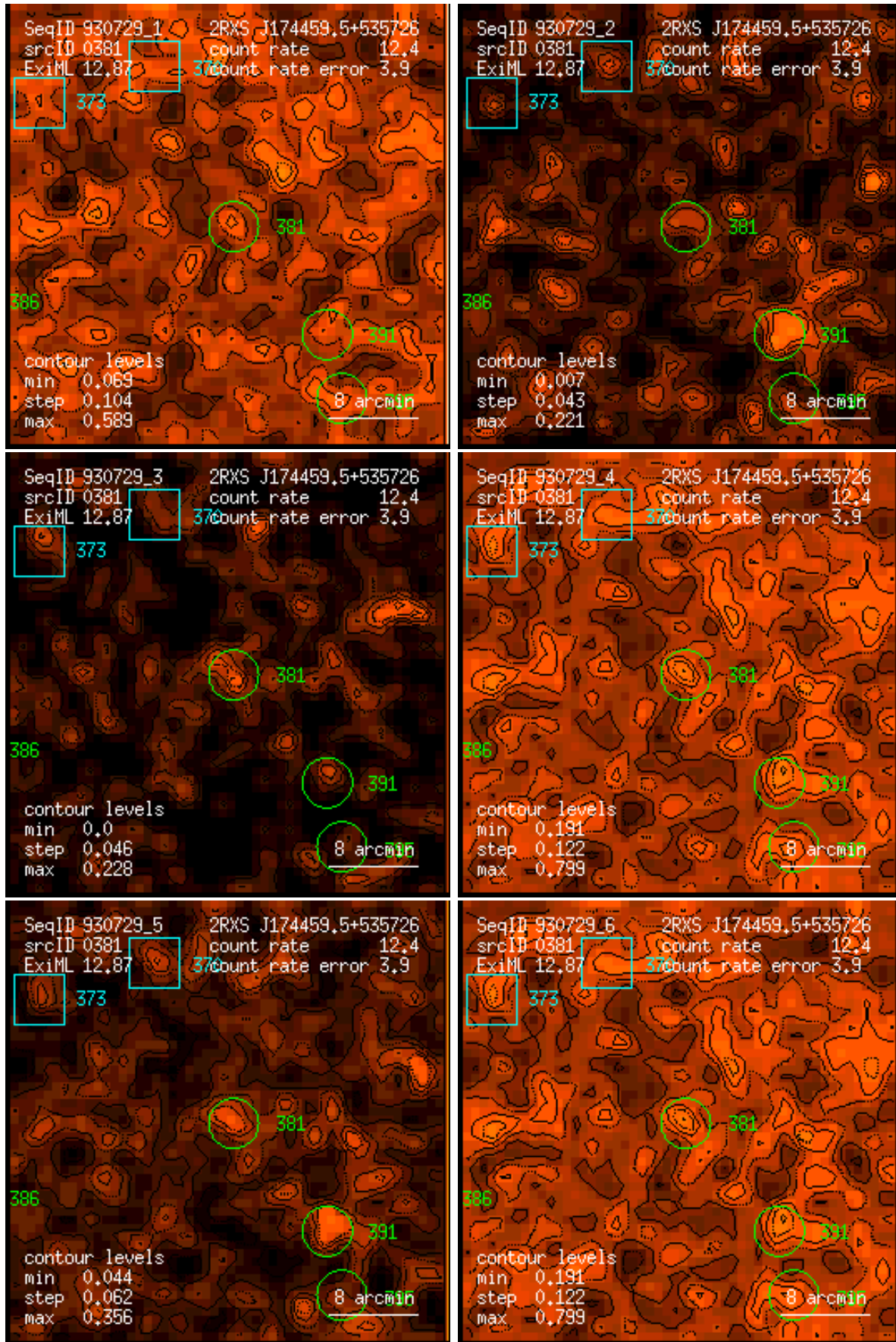
Figure 381: RASS 930729: detection 0381: band rate images, Gaussian filter: (1) PSPC channels 11 – 41, (2) 52 – 90, (3) 91 – 201, (4) 11 – 235, (5) 52 – 201, (6) 11 – 201. Broad band rates in counts/ks. Band rate contour levels in counts/ks/arcmin 2 .
