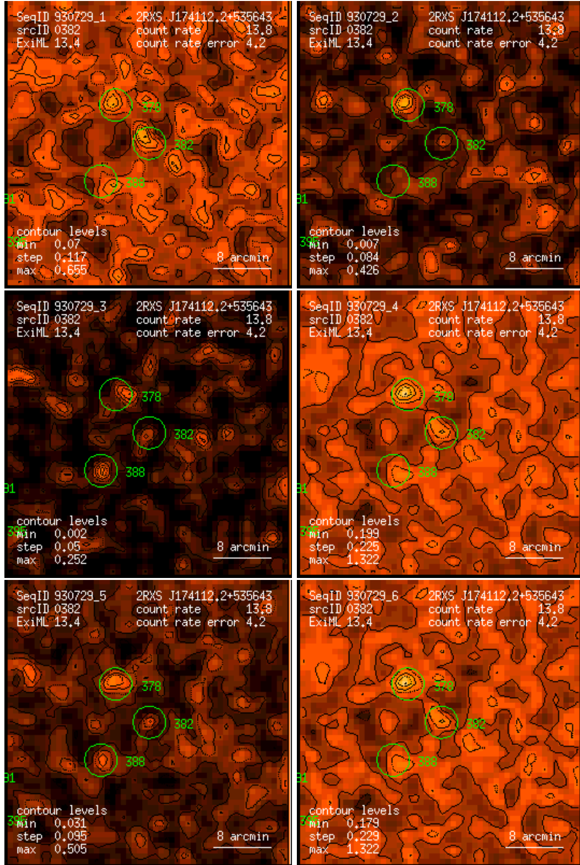
Figure 382: RASS 930729: detection 0382: band rate images, Gaussian filter: (1) PSPC channels 11 – 41, (2) 52 – 90, (3) 91 – 201, (4) 11 – 235, (5) 52 – 201, (6) 11 – 201. Broad band rates in counts/ks. Band rate contour levels in counts/ks/arcmin 2 .
