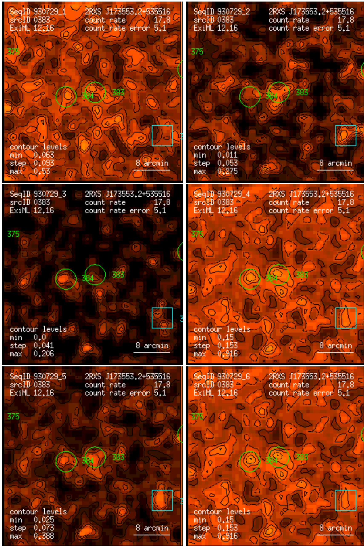
Figure 383: RASS 930729: detection 0383: band rate images, Gaussian filter: (1) PSPC channels 11 – 41, (2) 52 – 90, (3) 91 – 201, (4) 11 – 235, (5) 52 – 201, (6) 11 – 201. Broad band rates in counts/ks. Band rate contour levels in counts/ks/arcmin 2 .
