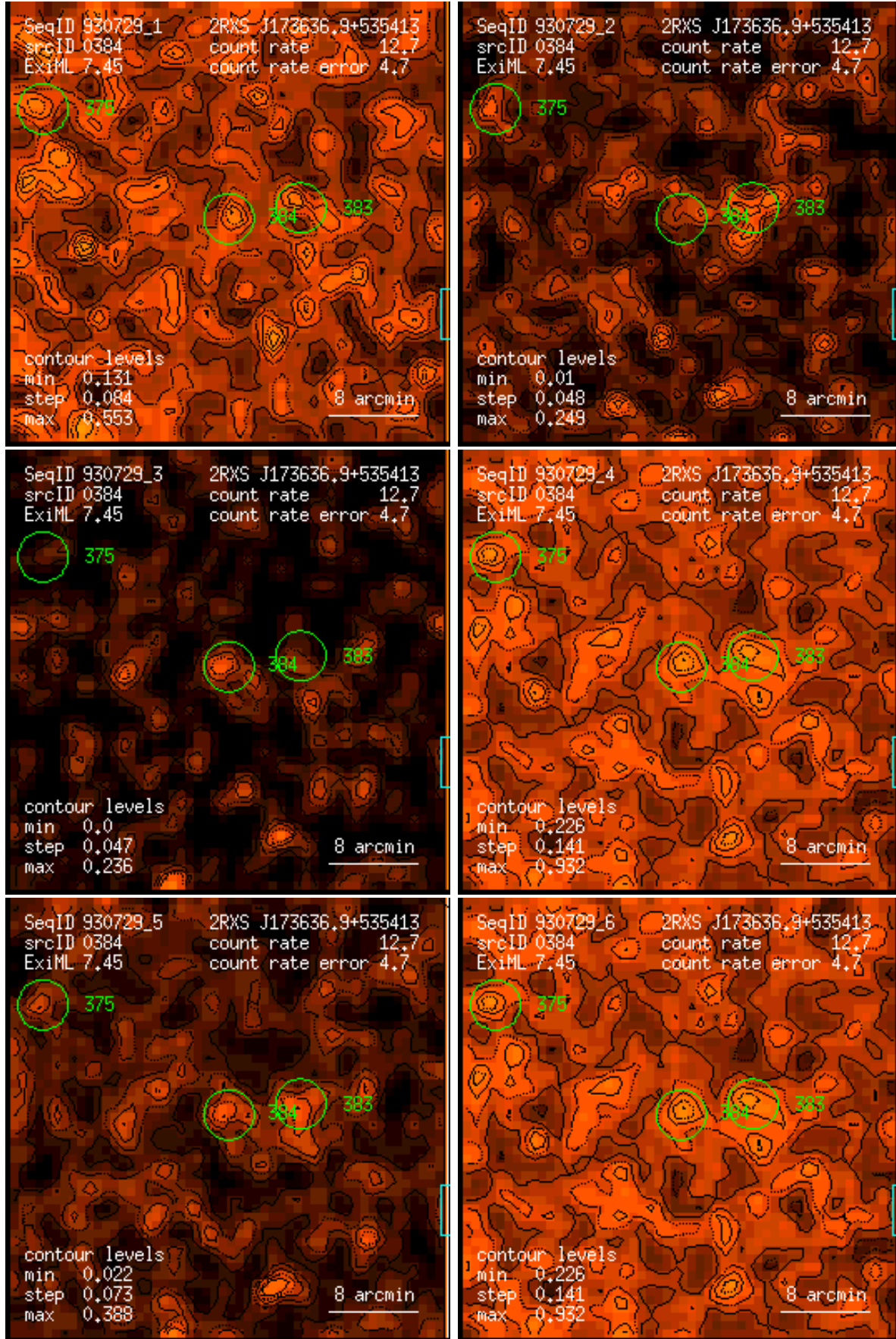
Figure 384: RASS 930729: detection 0384: band rate images, Gaussian filter: (1) PSPC channels 11 – 41, (2) 52 – 90, (3) 91 – 201, (4) 11 – 235, (5) 52 – 201, (6) 11 – 201. Broad band rates in counts/ks. Band rate contour levels in counts/ks/arcmin 2 .
