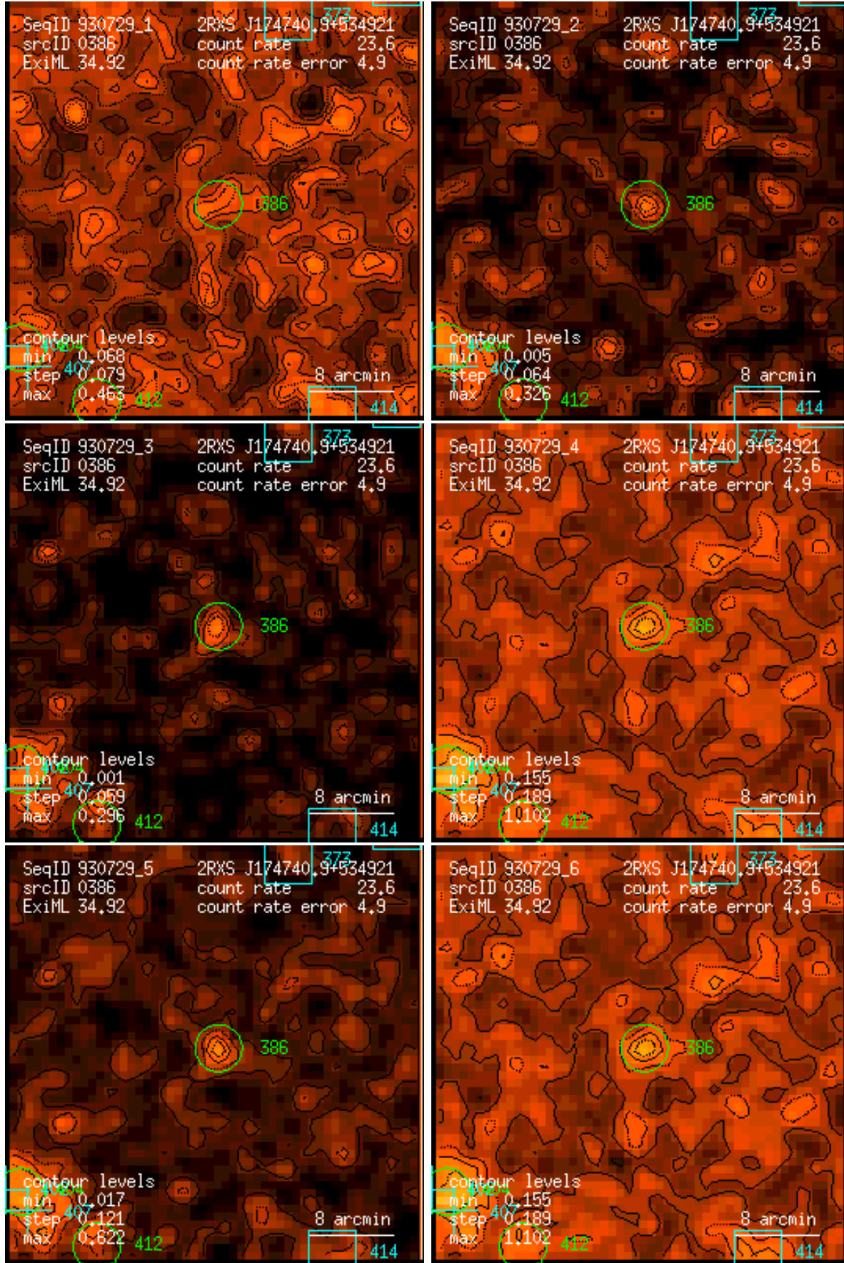
Figure 386: RASS 930729: detection 0386: band rate images, Gaussian filter: (1) PSPC channels 11 – 41, (2) 52 – 90, (3) 91 – 201, (4) 11 – 235, (5) 52 – 201, (6) 11 – 201. Broad band rates in counts/ks. Band rate contour levels in counts/ks/arcmin 2 .
