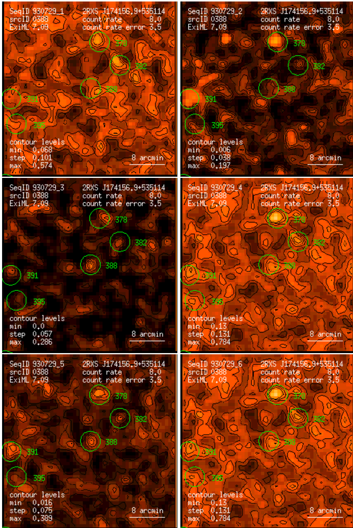
Figure 388: RASS 930729: detection 0388: band rate images, Gaussian filter: (1) PSPC channels 11 – 41, (2) 52 – 90, (3) 91 – 201, (4) 11 – 235, (5) 52 – 201, (6) 11 – 201. Broad band rates in counts/ks. Band rate contour levels in counts/ks/arcmin 2 .
