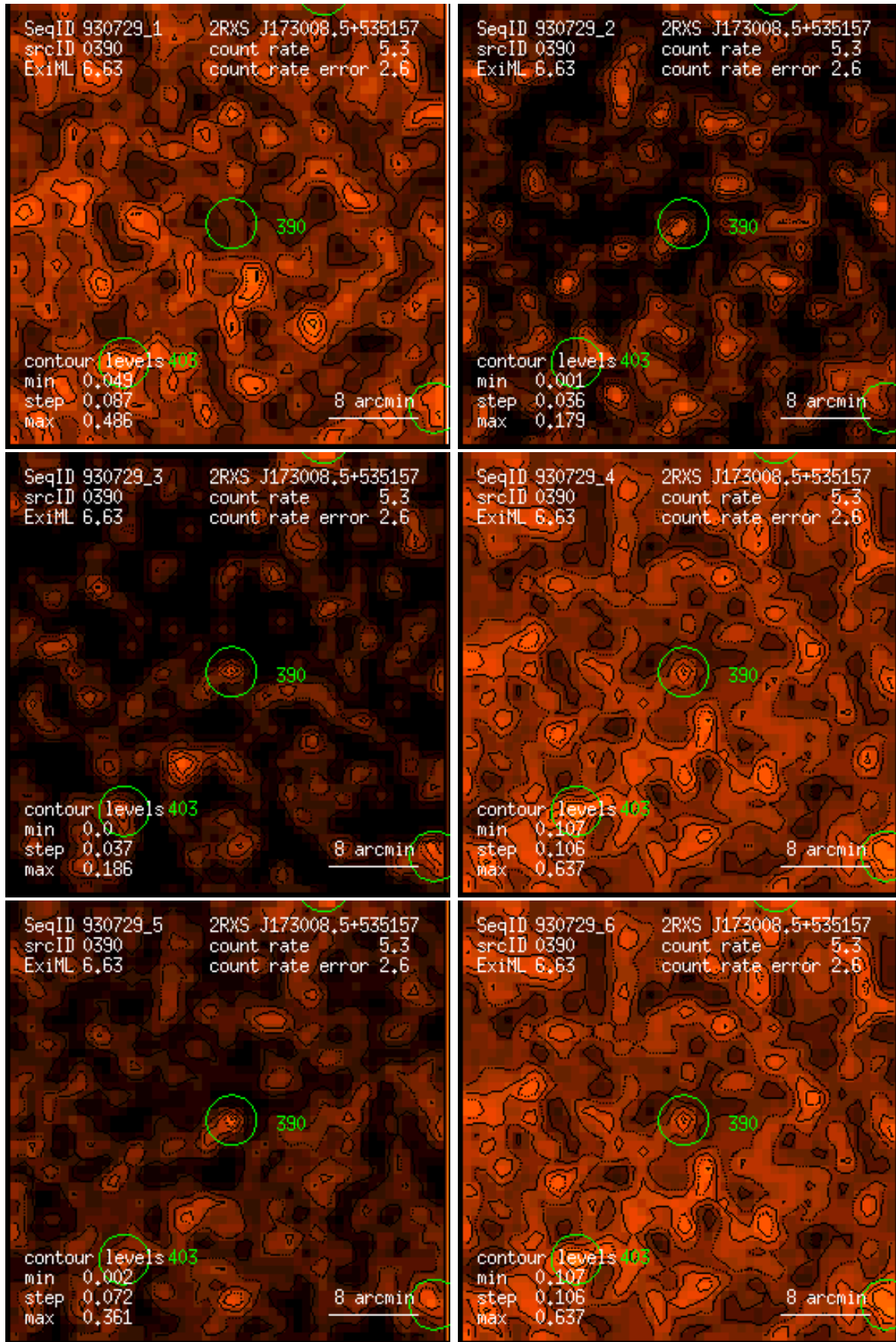
Figure 390: RASS 930729: detection 0390: band rate images, Gaussian filter: (1) PSPC channels 11 – 41, (2) 52 – 90, (3) 91 – 201, (4) 11 – 235, (5) 52 – 201, (6) 11 – 201. Broad band rates in counts/ks. Band rate contour levels in counts/ks/arcmin 2 .
