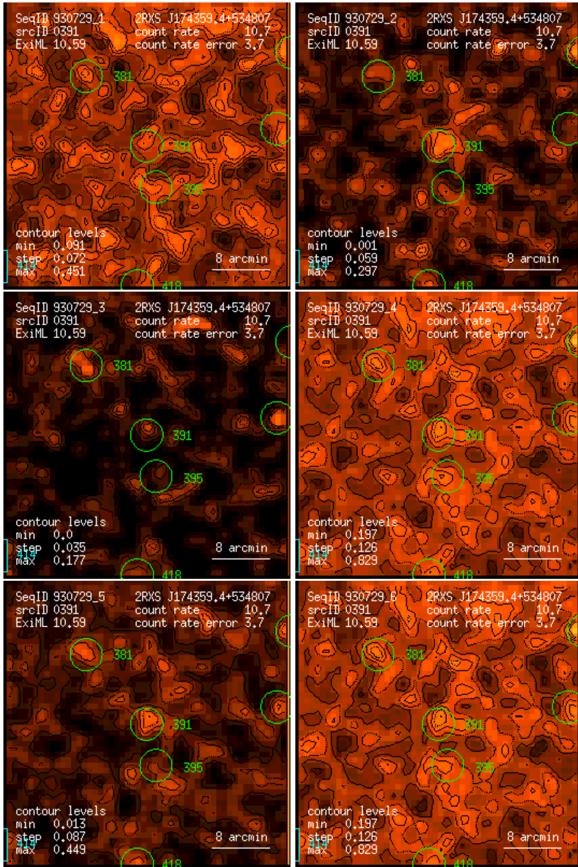
Figure 391: RASS 930729: detection 0391: band rate images, Gaussian filter: (1) PSPC channels 11 – 41, (2) 52 – 90, (3) 91 – 201, (4) 11 – 235, (5) 52 – 201, (6) 11 – 201. Broad band rates in counts/ks. Band rate contour levels in counts/ks/arcmin 2 .
