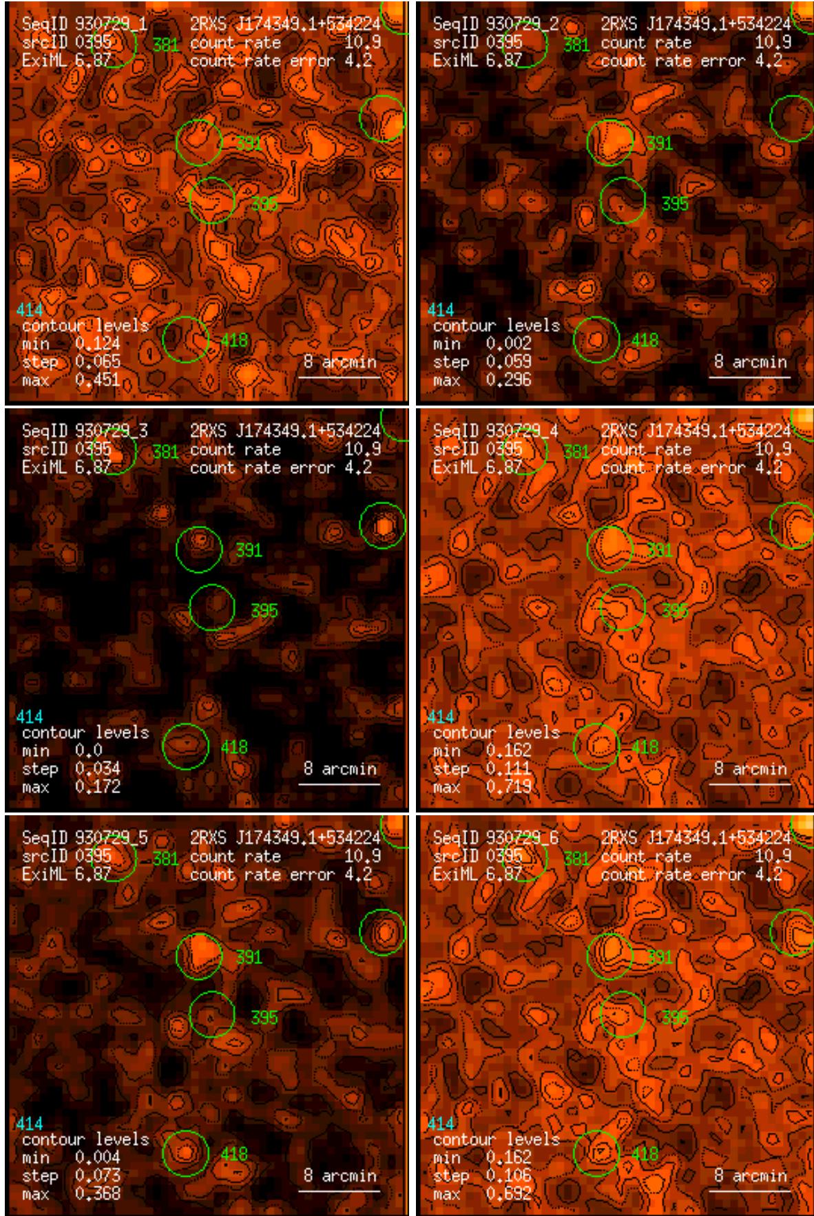
Figure 395: RASS 930729: detection 0395: band rate images, Gaussian filter: (1) PSPC channels 11 – 41, (2) 52 – 90, (3) 91 – 201, (4) 11 – 235, (5) 52 – 201, (6) 11 – 201. Broad band rates in counts/ks. Band rate contour levels in counts/ks/arcmin 2 .
